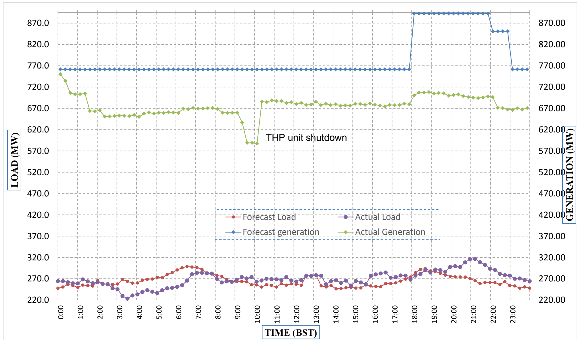
Forecast Generation & Load with Actual Generation & Load (19-Jun-2019).
