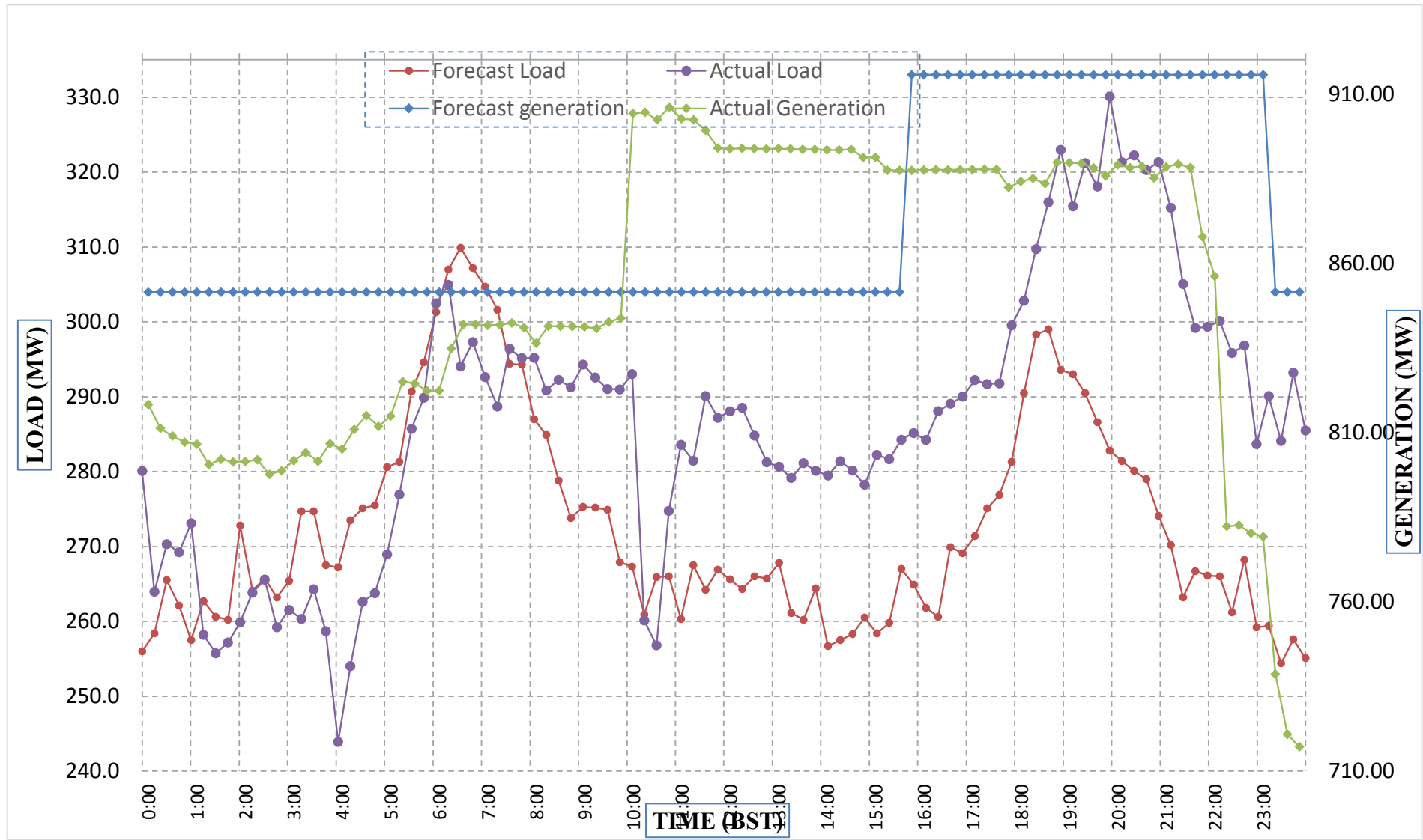
Forecast Generation & Load with Actual Generation & Load (09-May-2019).
