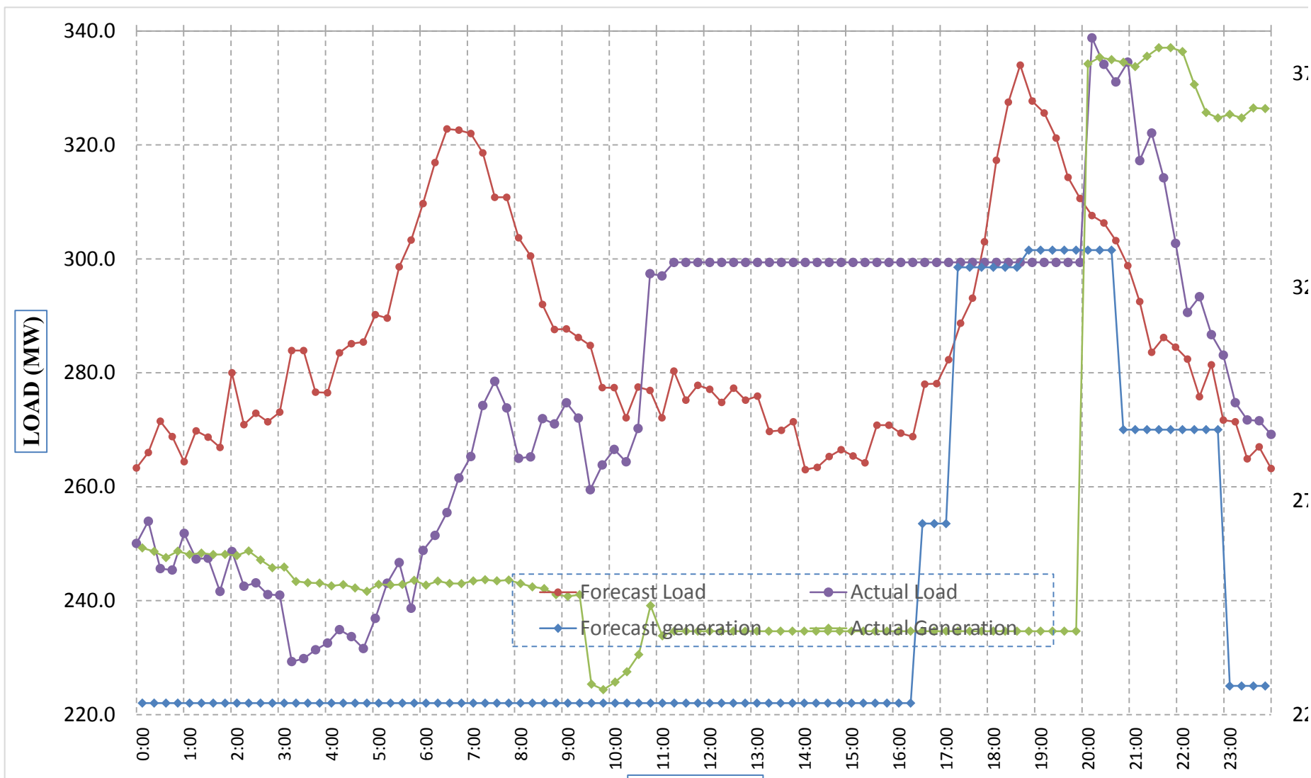
Forecast Generation & Load with Actual Generation & Load (08-Feb-2019).
