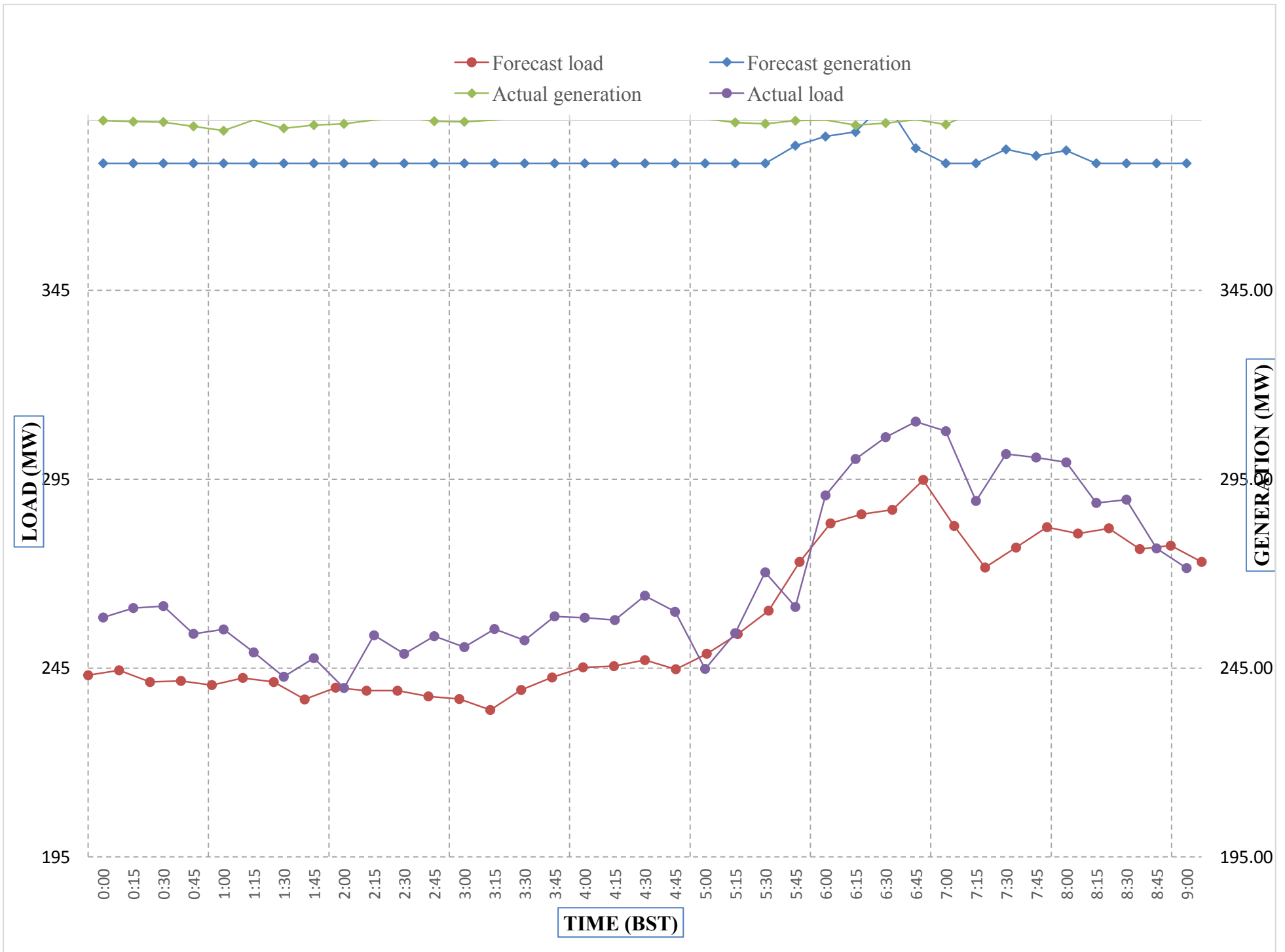
Forecast Generation & Load with Actual Generation & Load of Today from 00:00hrs to 09:00hrs(30-Apr-2018).
