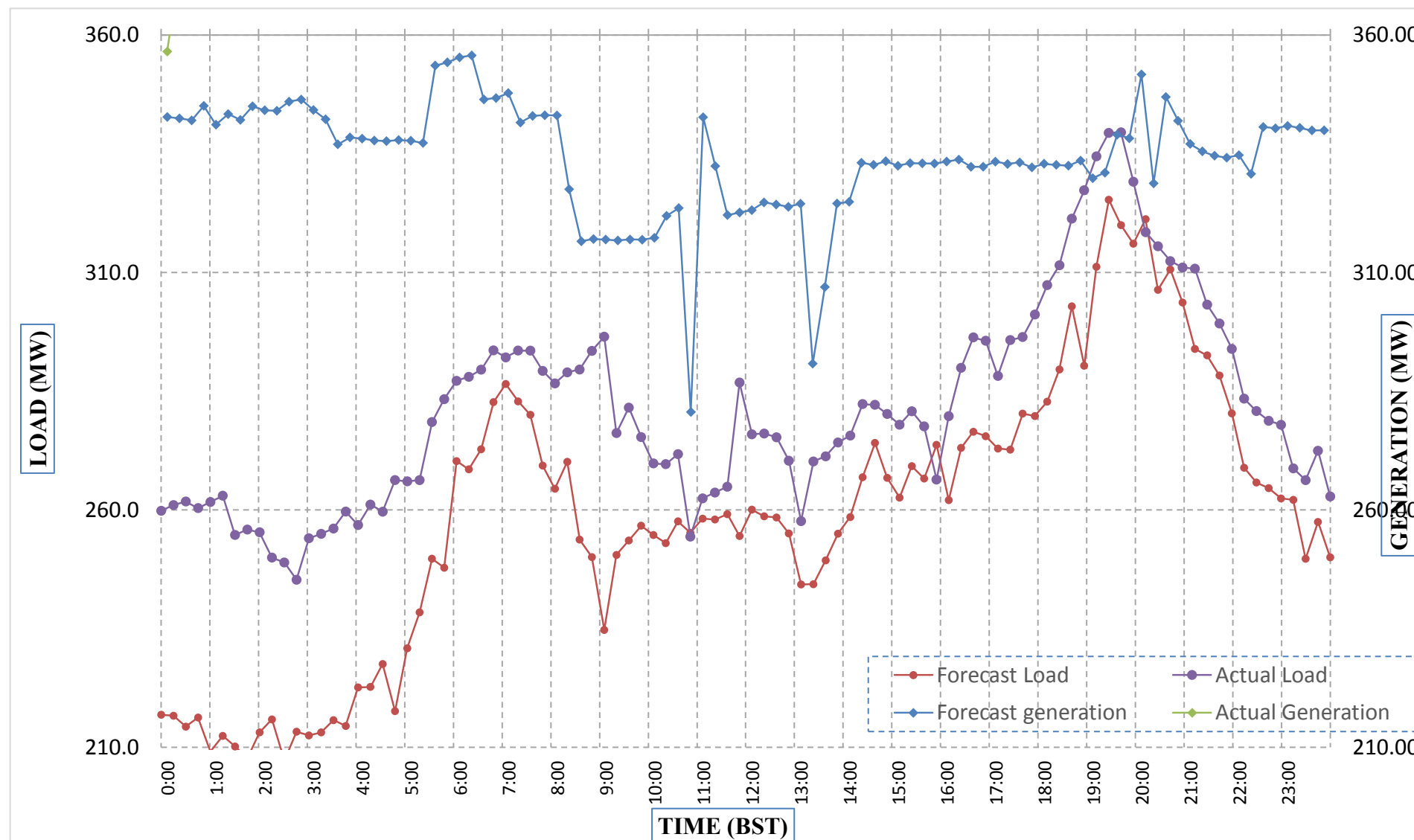
Forecast Generation & Load with Actual Generation & Load (29-Apr-2018).
