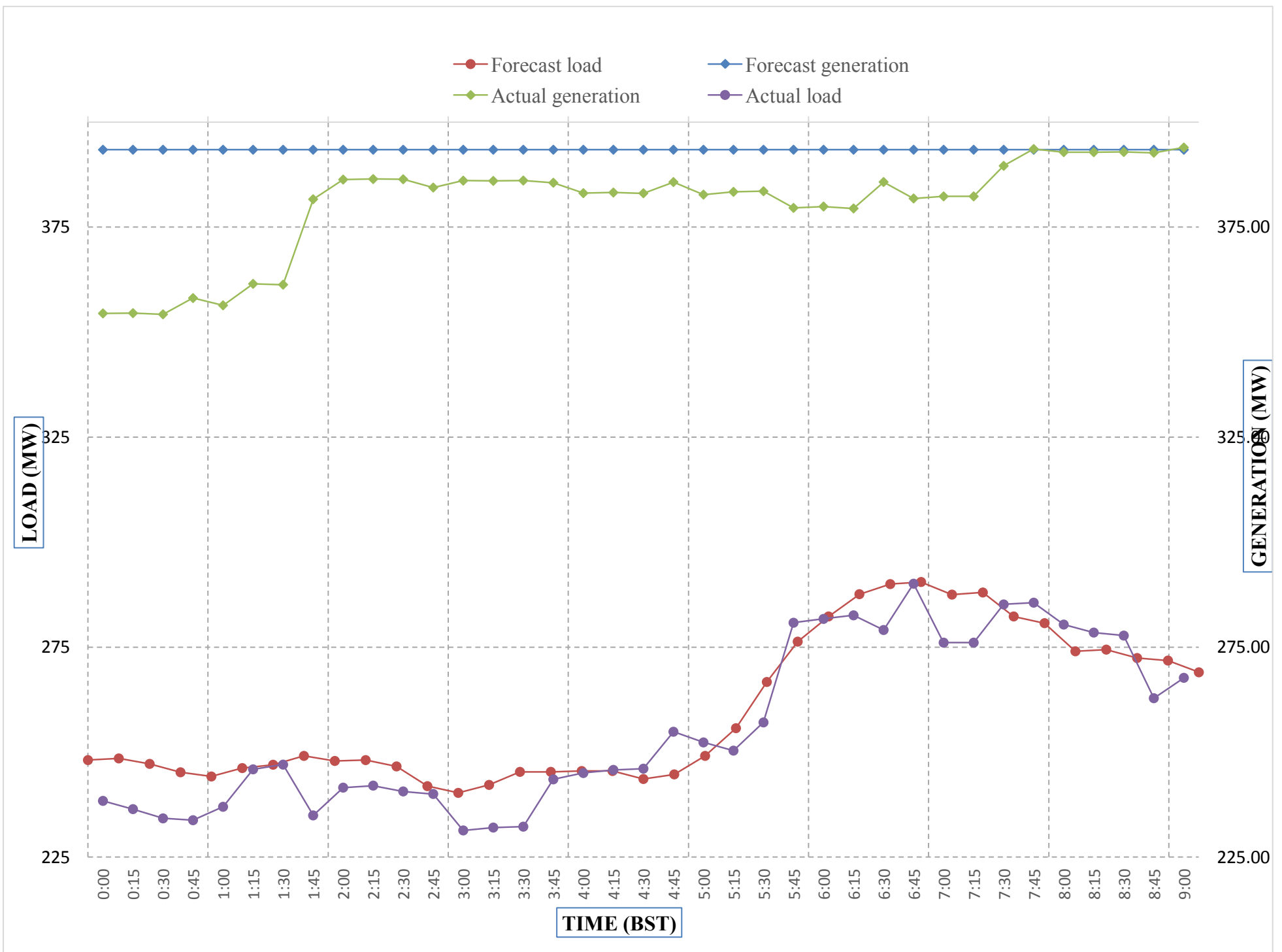
Forecast Generation & Load with Actual Generation & Load of Today from 00:00hrs to 09:00hrs(25-Apr-2018).
