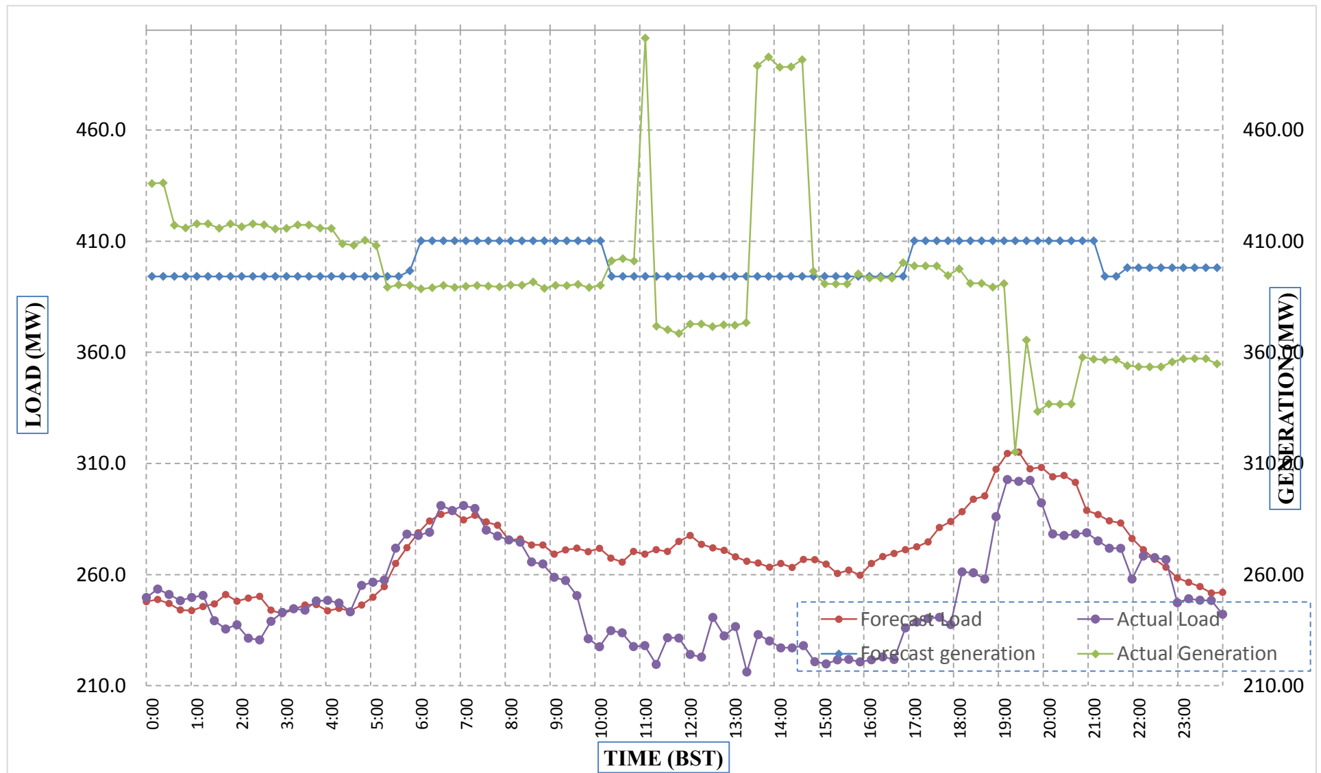
Forecast Generation & Load with Actual Generation & Load (24-Apr-2018).
