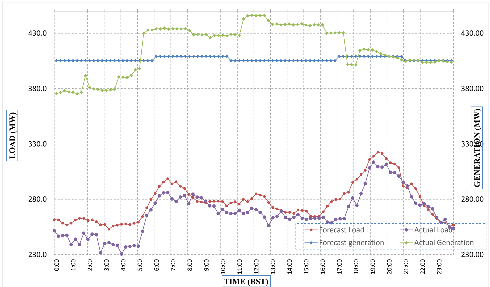
Forecast Generation & Load with Actual Generation & Load (22-Apr-2018).
