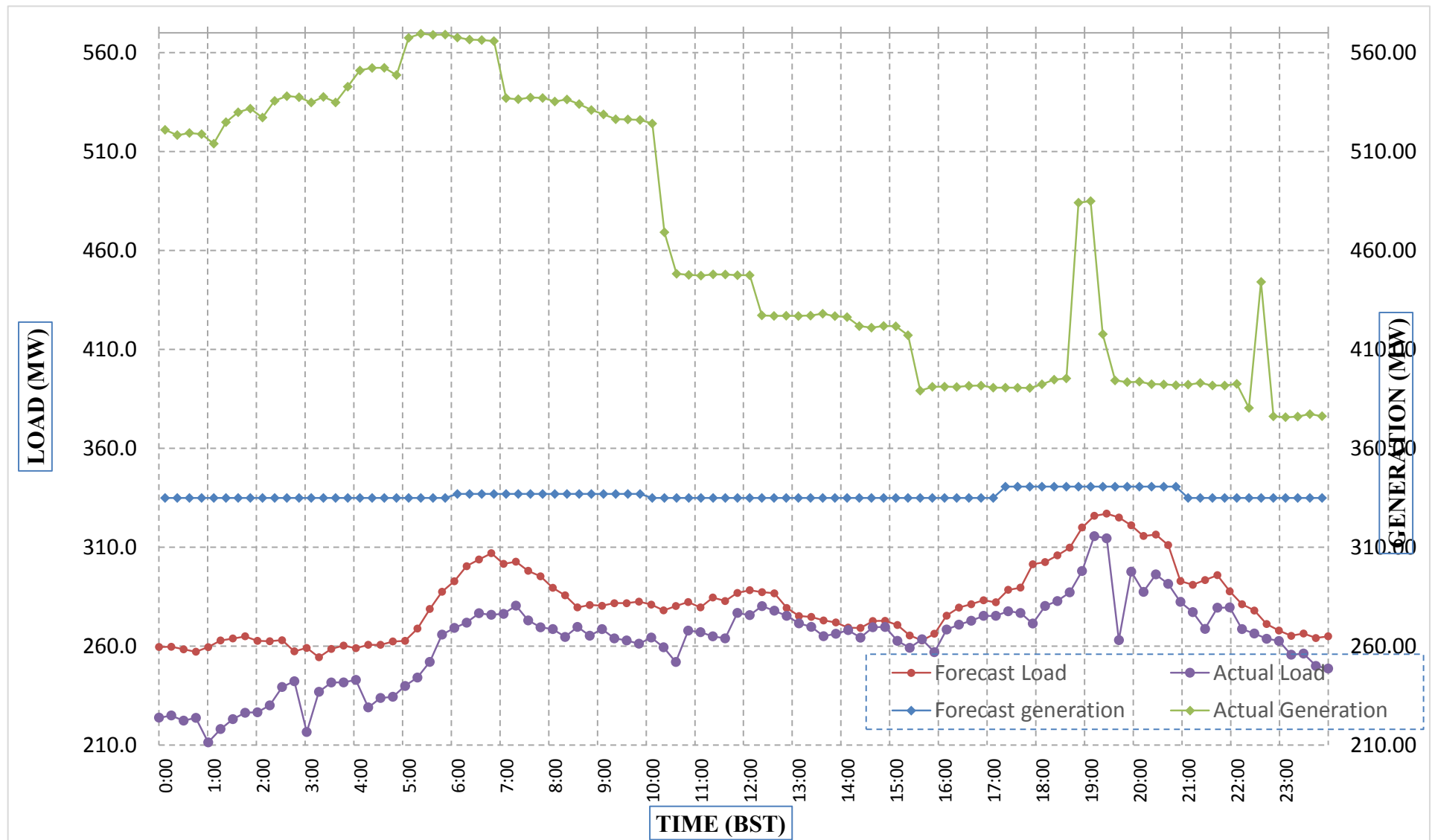
Forecast Generation & Load with Actual Generation & Load (21-Apr-2018).
