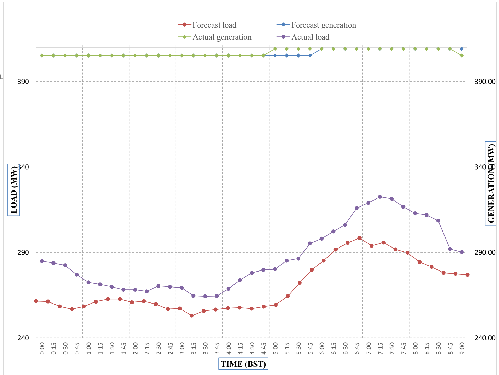
Forecast Generation & Load with Actual Generation & Load of Today from 00:00hrs to 09:00hrs(22-Apr-2018).
