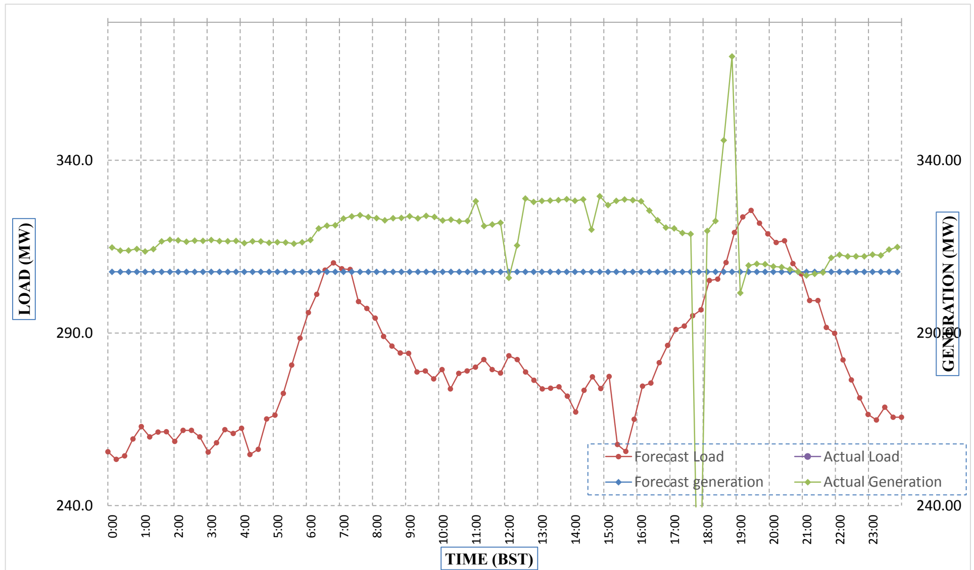
Forecast Generation & Load with Actual Generation & Load (16-Apr-2018).
