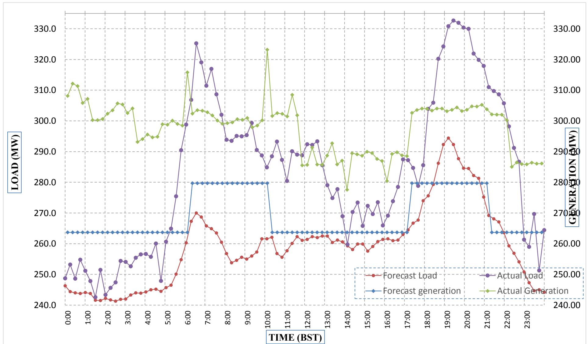
Forecast Generation & Load with Actual Generation & Load (04-Apr-2018).
