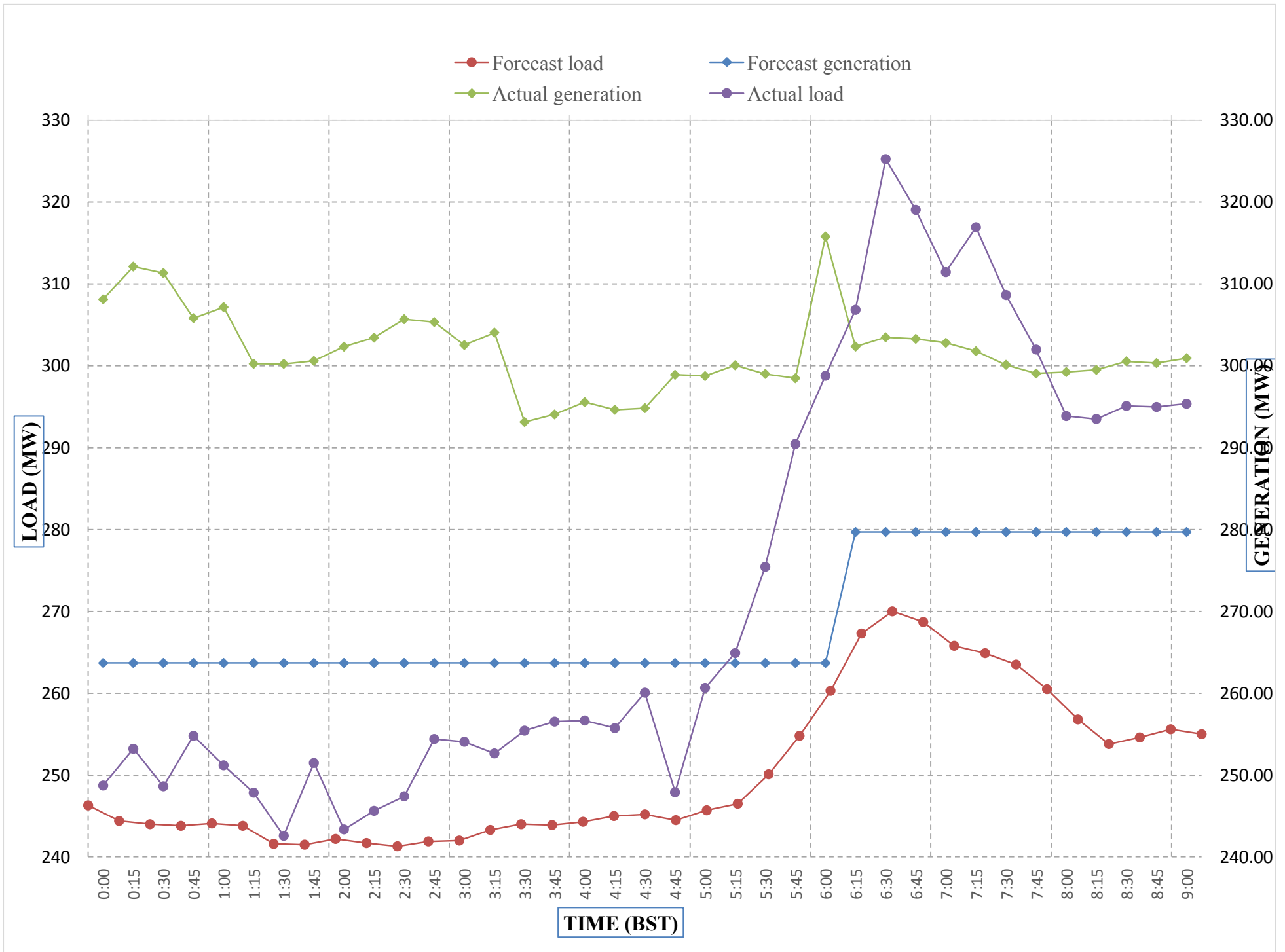
Forecast Generation & Load with Actual Generation & Load of Today from 00:00hrs to 09:00hrs(04-Apr-2018).
