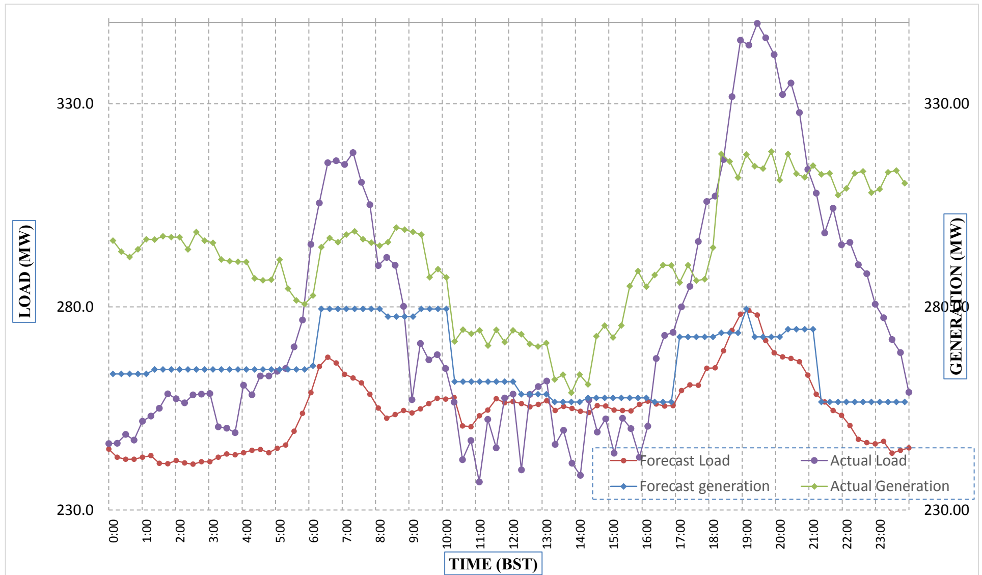
Forecast Generation & Load with Actual Generation & Load (03-Apr-2018).
