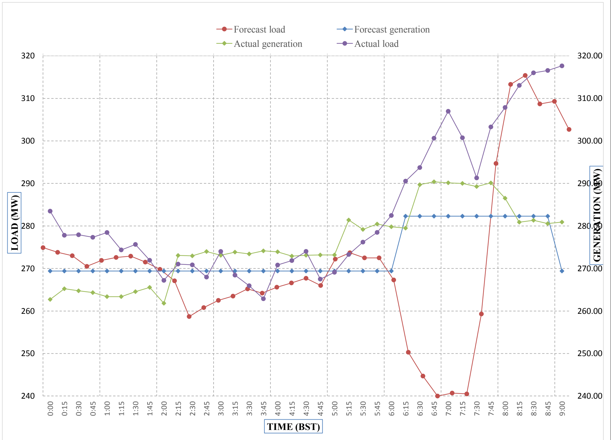
Forecast Generation & Load with Actual Generation & Load of Today from 00:00hrs to 09:00hrs(25-Feb-2018).
