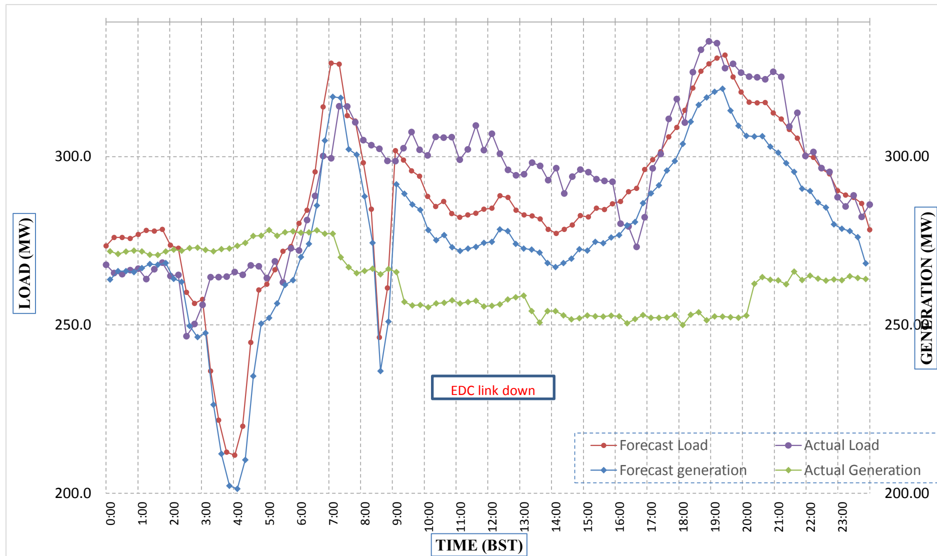
Forecast Generation & Load with Actual Generation & Load (20-Feb-2018).
