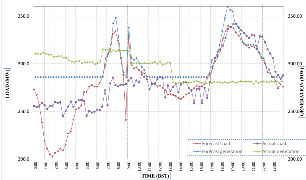
Forecast Generation & Load with Actual Generation & Load (04-Feb-2018).
