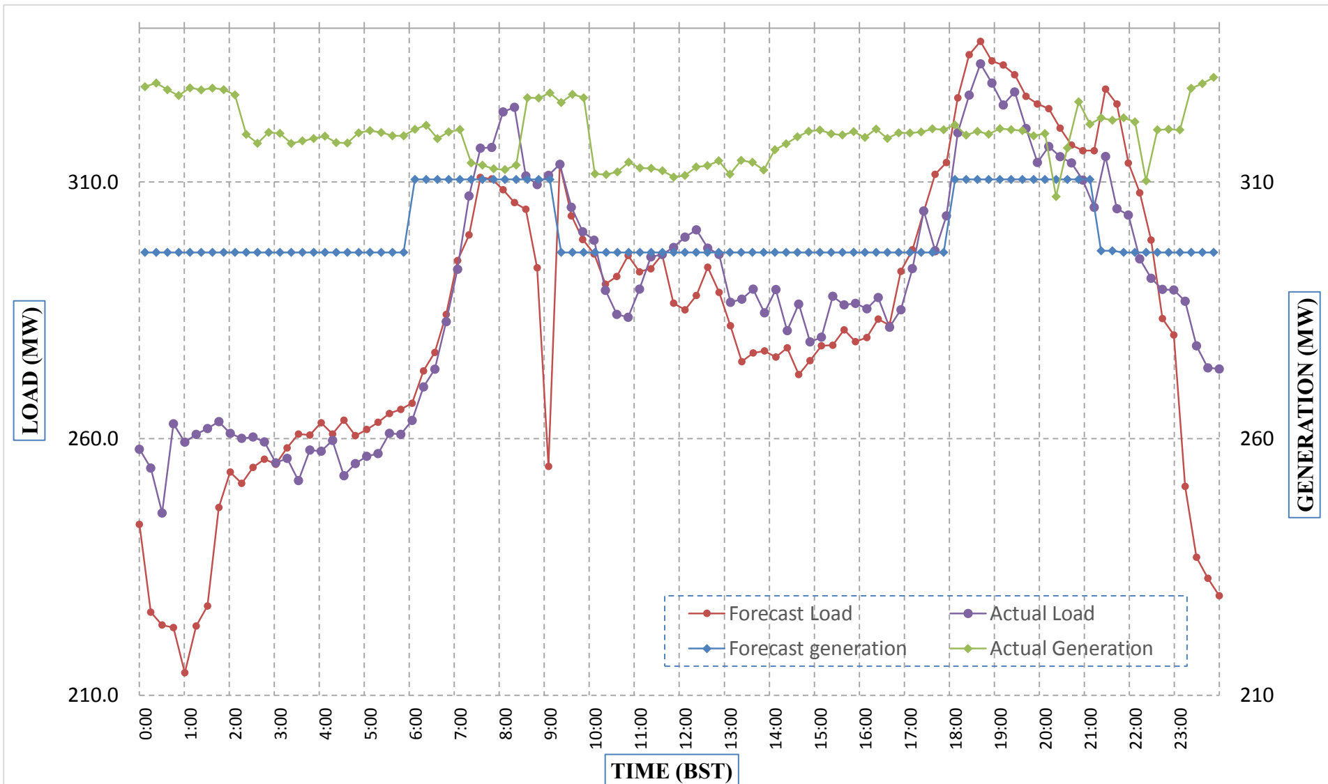
Forecast Generation & Load with Actual Generation & Load (28-Jan-2018).
