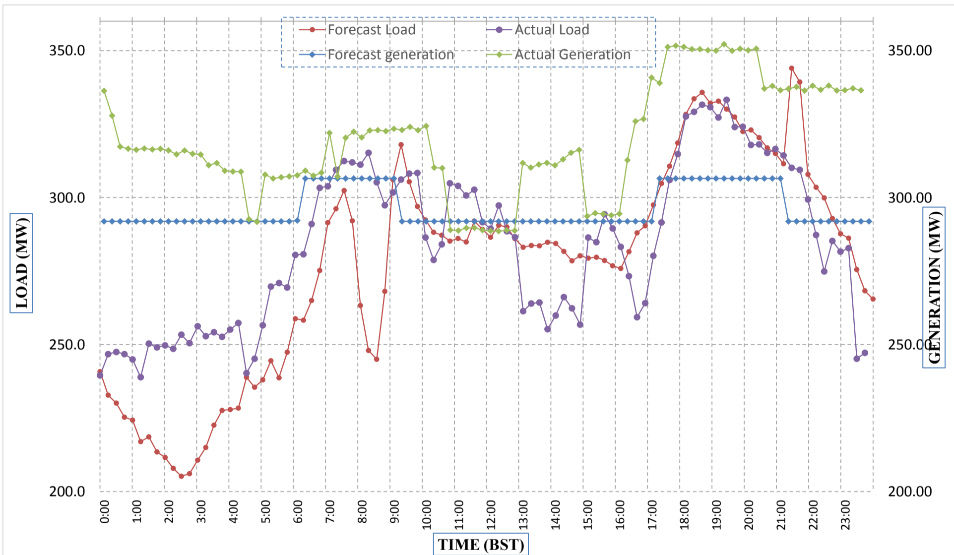
Forecast Generation & Load with Actual Generation & Load (22-Jan-2018).
