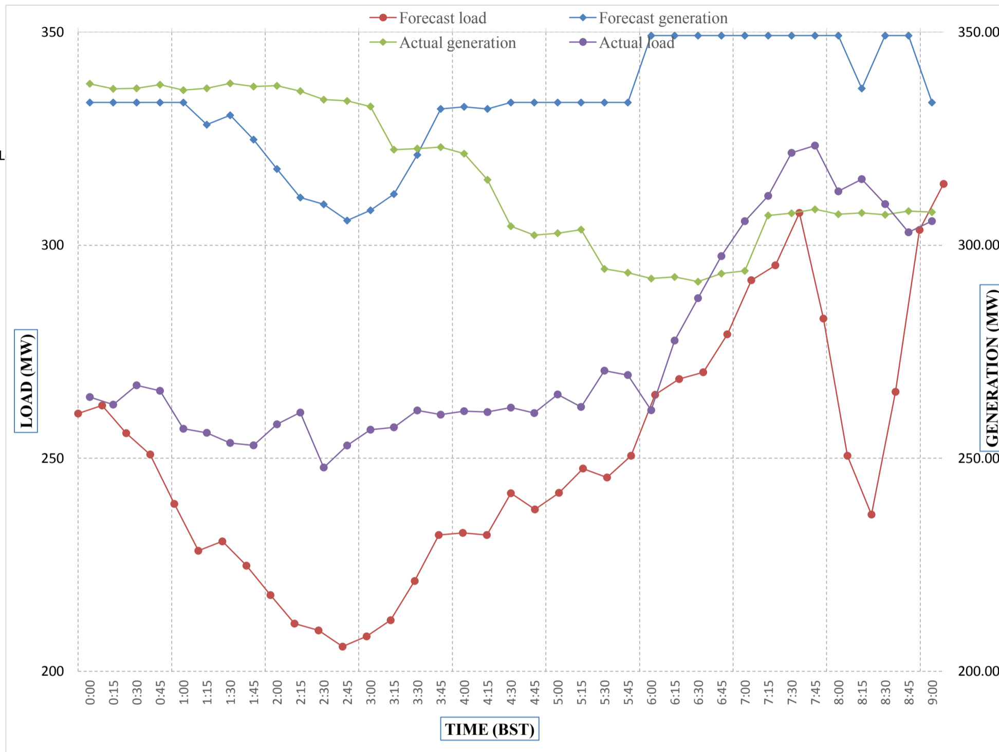
Forecast Generation & Load with Actual Generation & Load of Today from 00:00hrs to 09:00hrs(23-Jan-2018).
