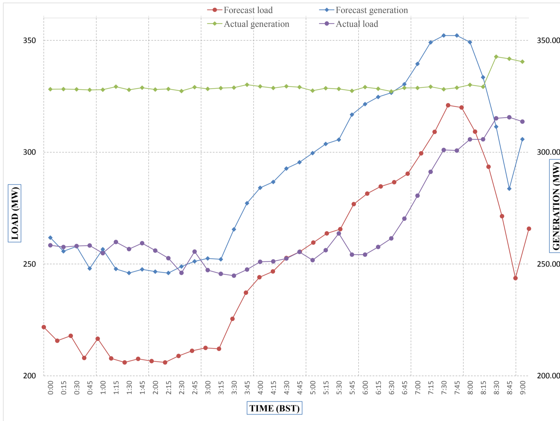
Forecast Generation & Load with Actual Generation & Load of Today from 00:00hrs to 09:00hrs(16-Jan-2018).
