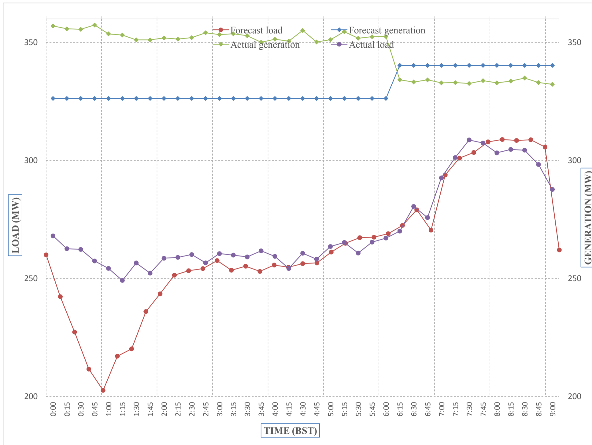
Forecast Generation & Load with Actual Generation & Load of Today from 00:00hrs to 09:00hrs(05-Jan-2018).
