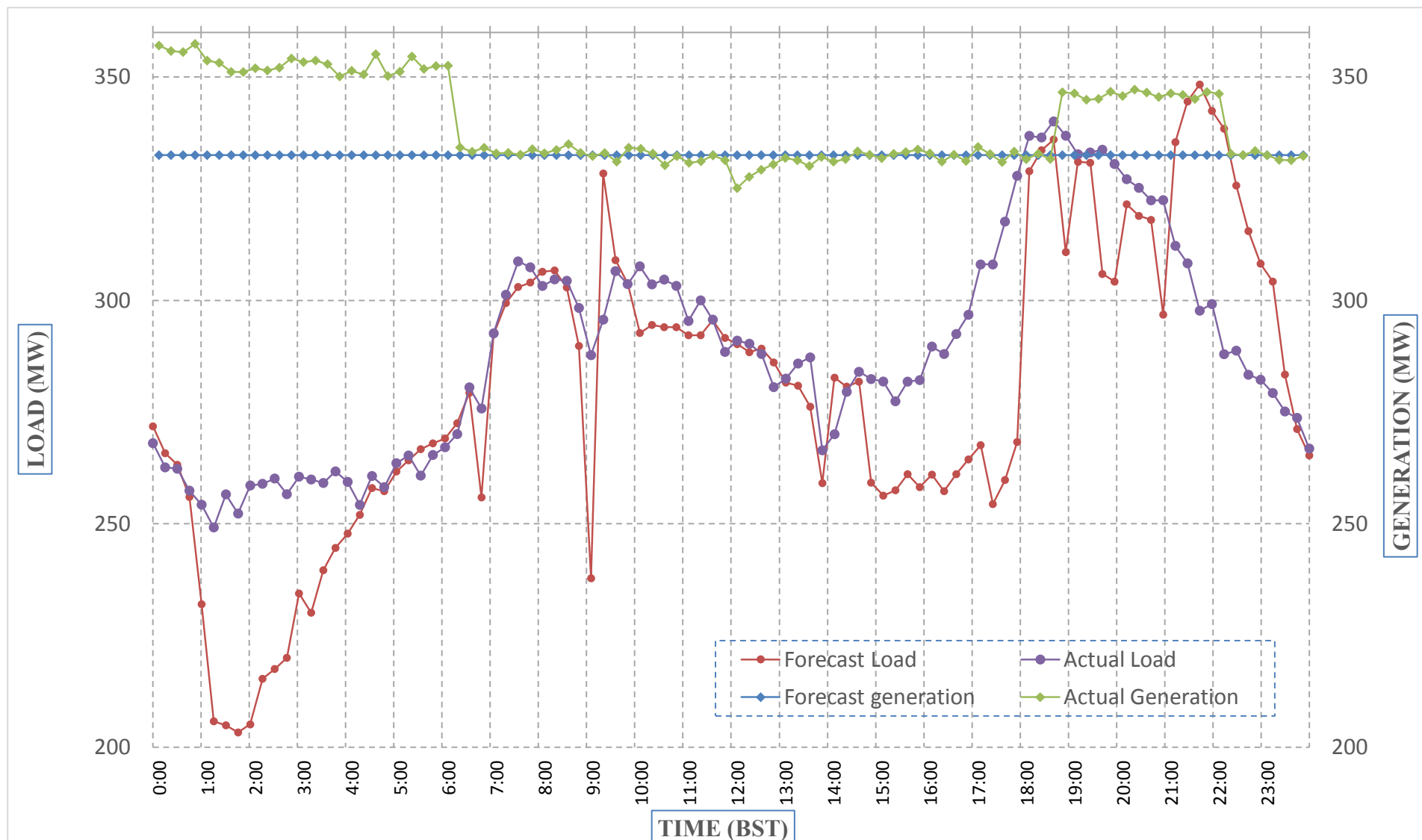
Forecast Generation & Load with Actual Generation & Load (04-Jan-2018).
