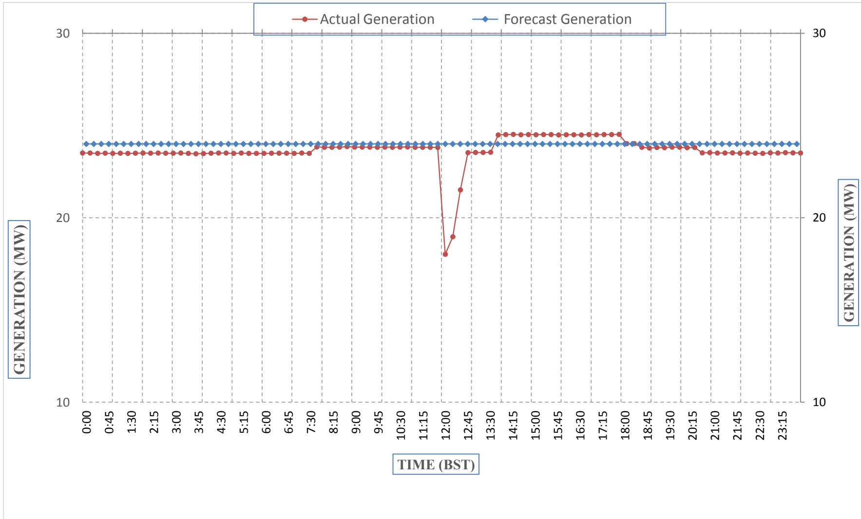
Scheduled Generation & Actual Generation of Dagachhu(04-Jan-2018).
