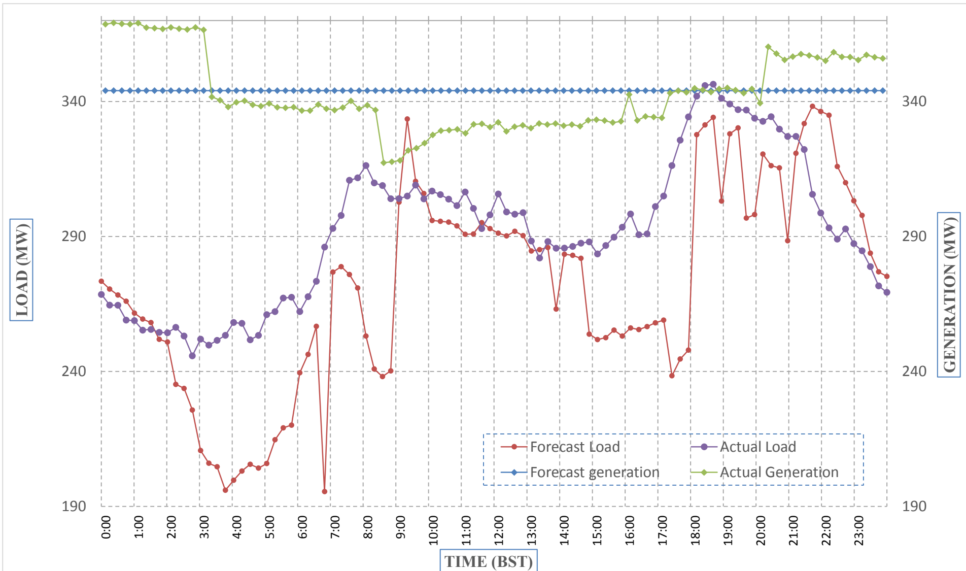
Forecast Generation & Load with Actual Generation & Load (03-Jan-2018).
