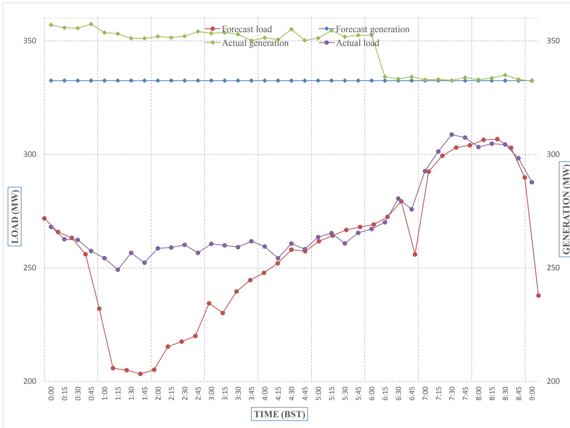
Forecast Generation & Load with Actual Generation & Load of Today from 00:00hrs to 09:00hrs(04-Jan-2018).
