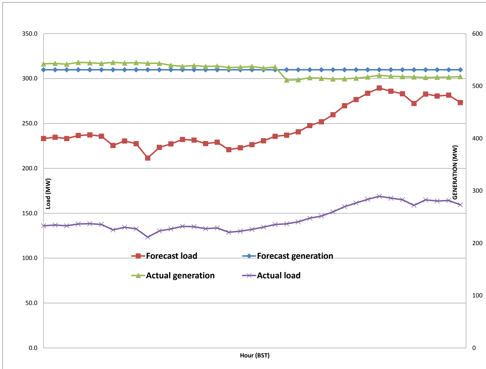
Forecast Generation & Load with Actual Generation & Load of Today from 00:00hrs to 09:00hrs(28-Nov-2017).
