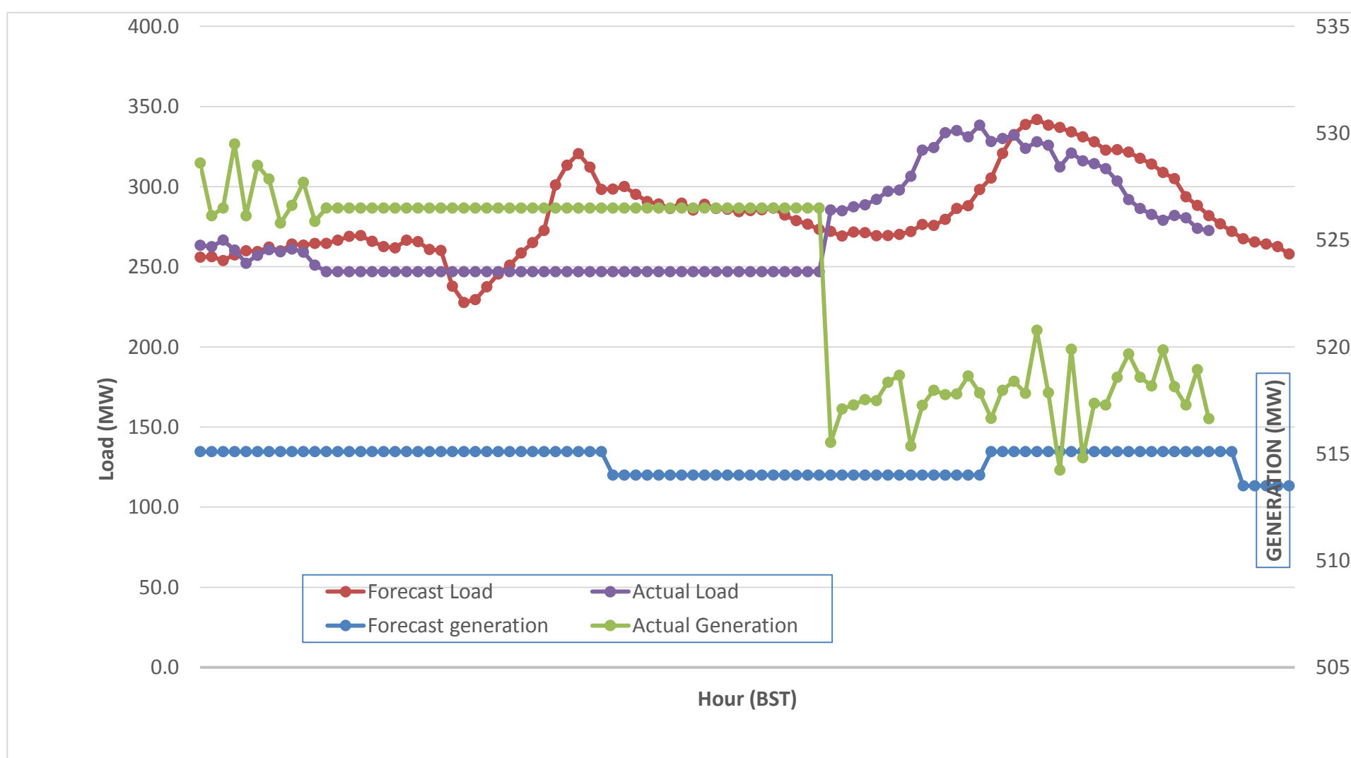
Forecast Generation & Load with Actual Generation & Load (26-Nov-2017).
