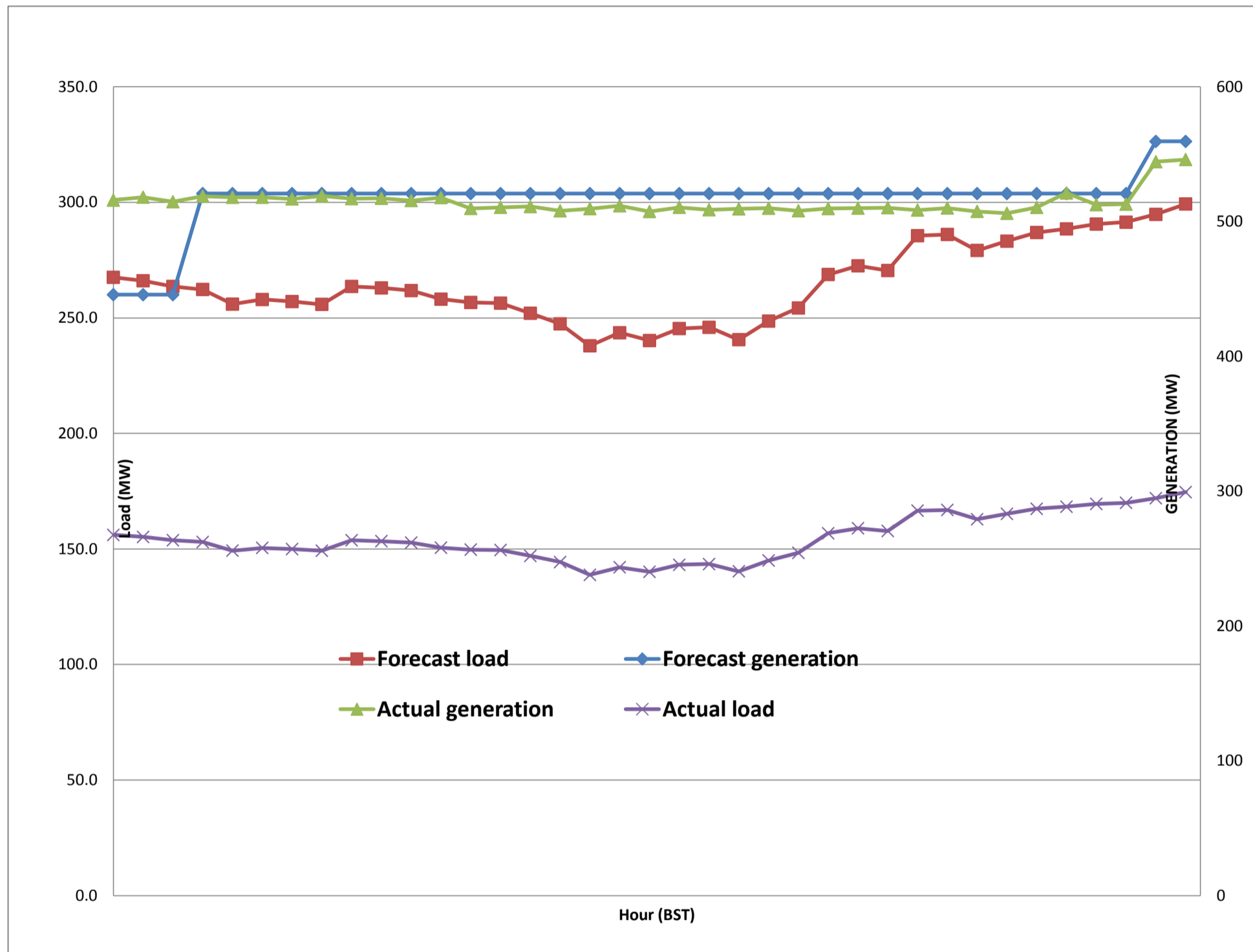
Forecast Generation & Load with Actual Generation & Load of Today from 00:00hrs to 09:00hrs(27-Nov-2017).
