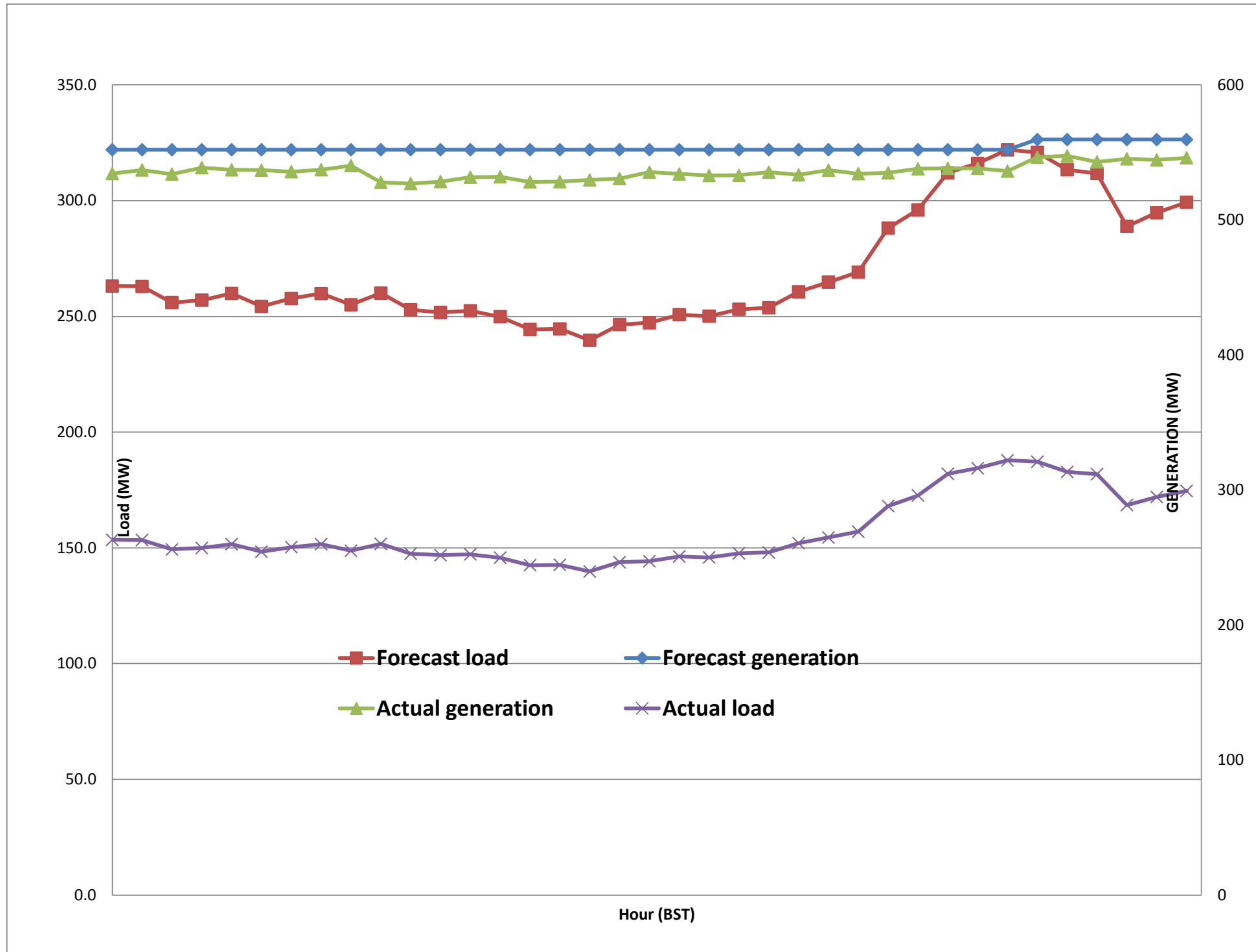
Forecast Generation & Load with Actual Generation & Load of Today from 00:00hrs to 09:00hrs(22-Nov-2017).
