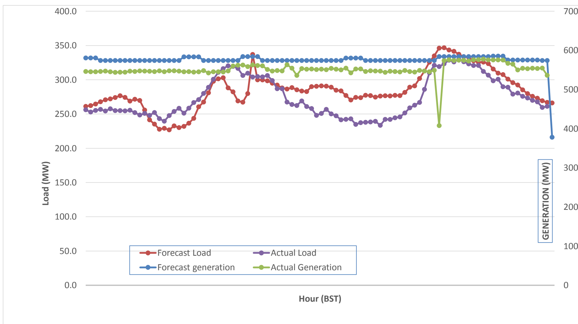
Forecast Generation & Load with Actual Generation & Load (21-Nov-2017).
