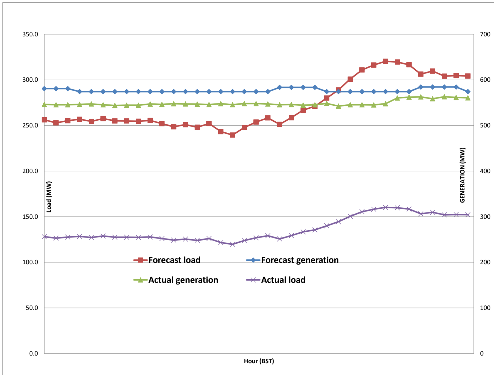
Forecast Generation & Load with Actual Generation & Load of Today from 00:00hrs to 09:00hrs(21-Nov-2017).
