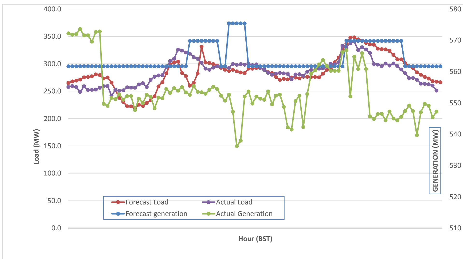
Forecast Generation & Load with Actual Generation & Load (20-Nov-2017).
