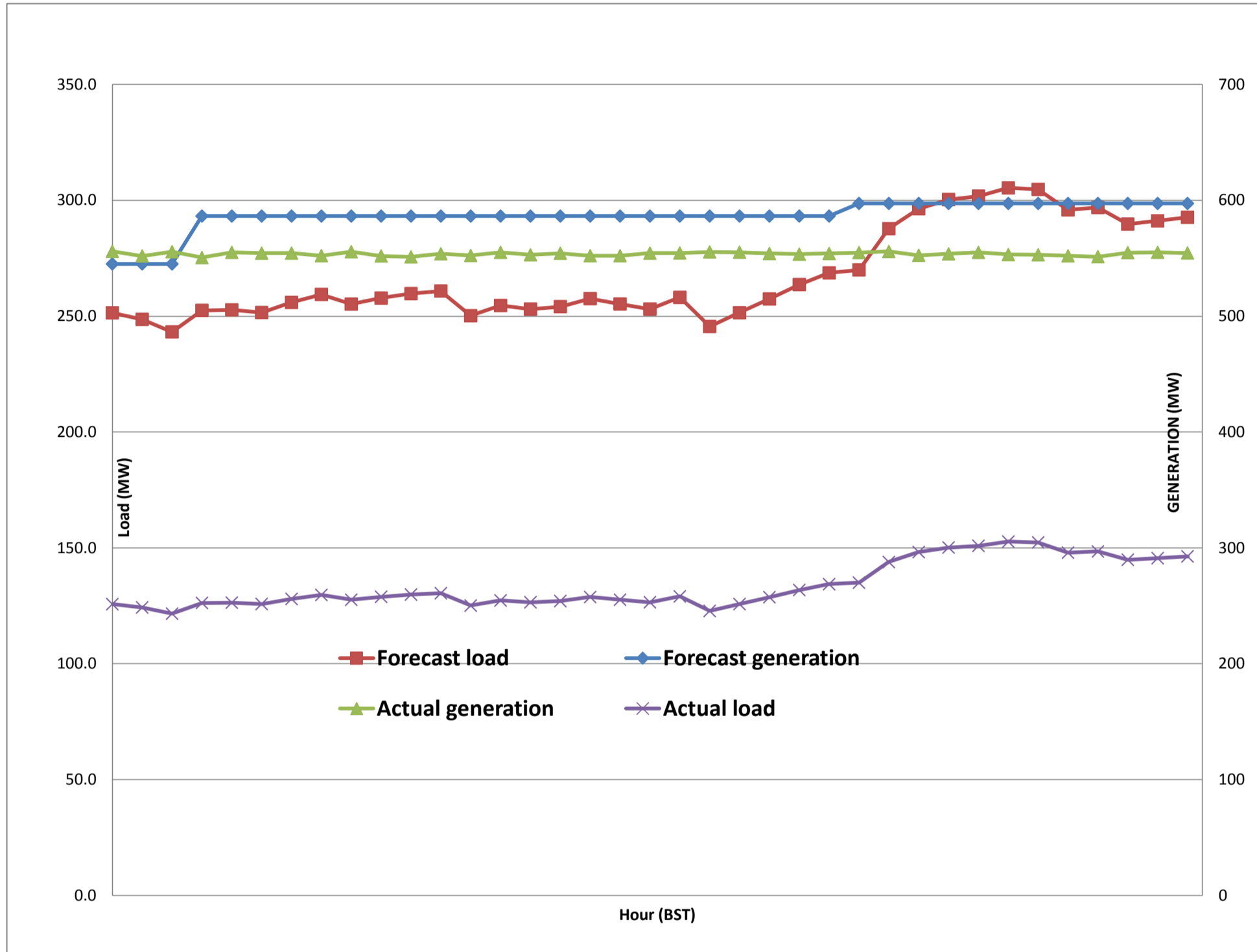
Forecast Generation & Load with Actual Generation & Load of Today from 00:00hrs to 09:00hrs(19-Nov-2017).
