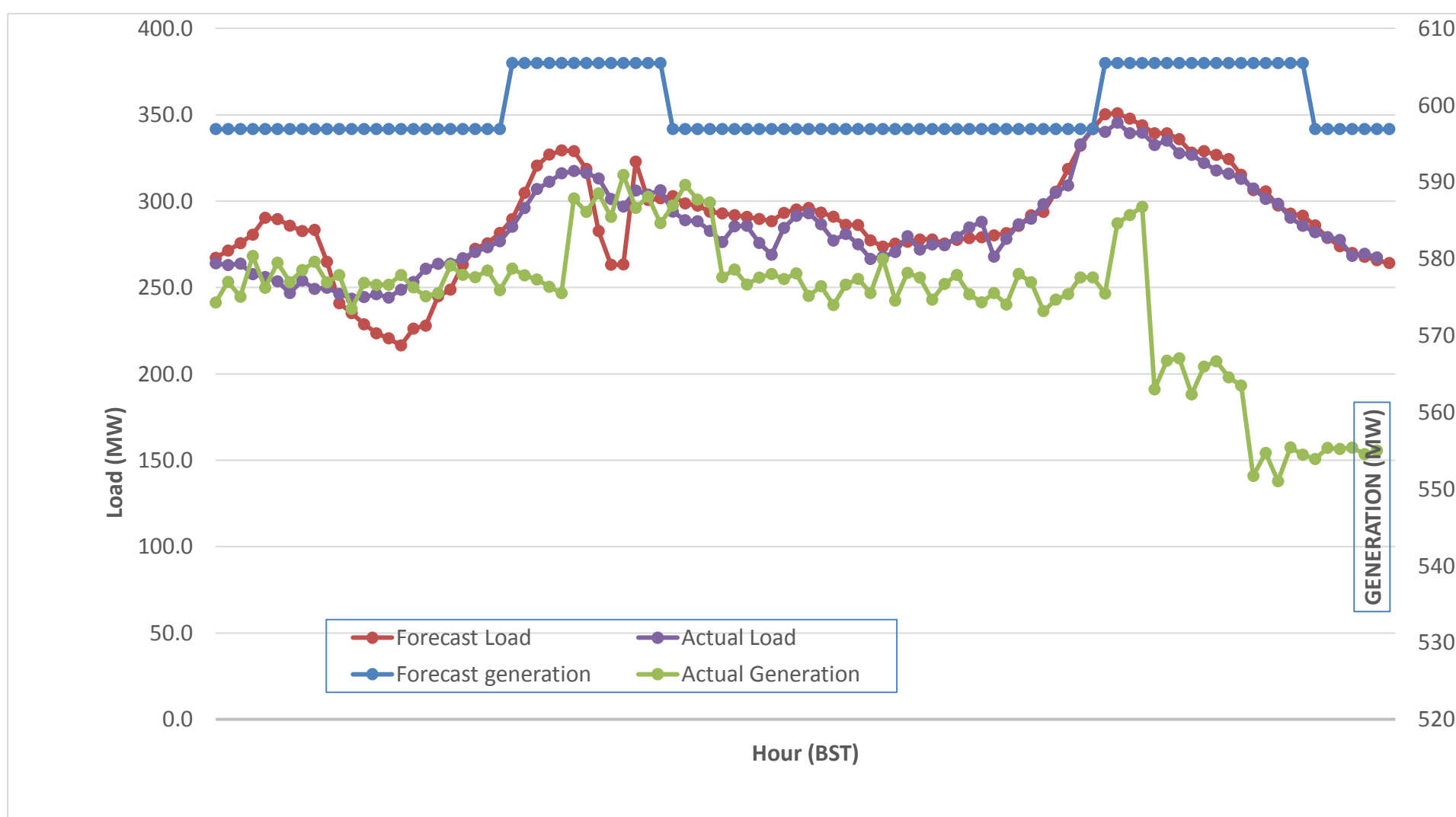
Forecast Generation & Load with Actual Generation & Load (18-Nov-2017).
