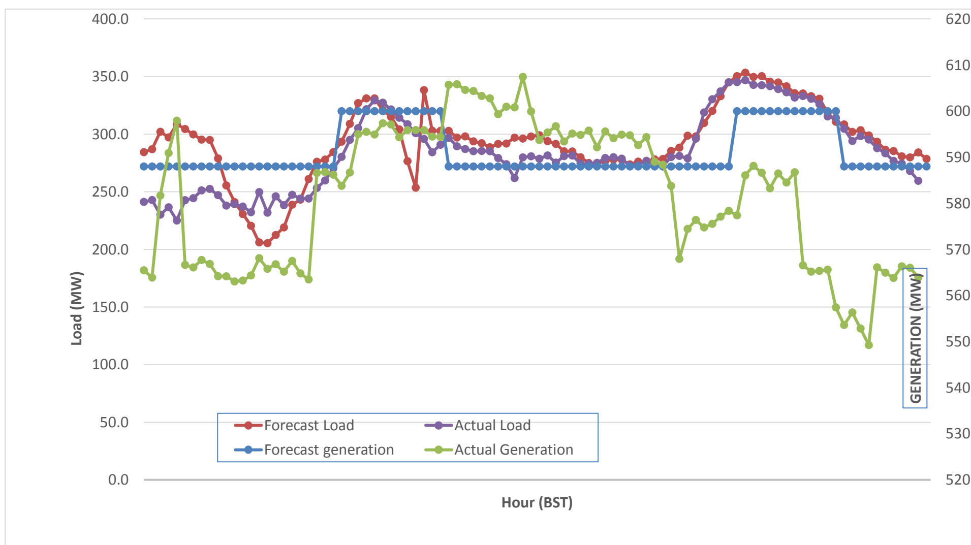
Forecast Generation & Load with Actual Generation & Load (16-Nov-2017).
