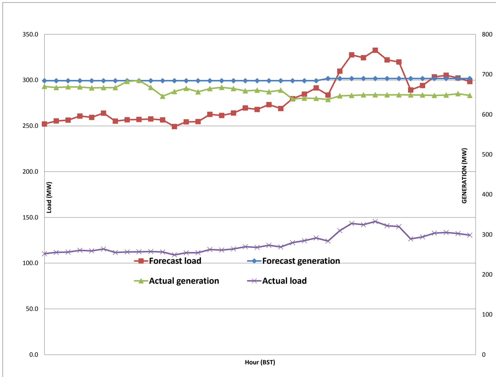
Forecast Generation & Load with Actual Generation & Load of Today from 00:00hrs to 09:00hrs(08-Nov-2017).
