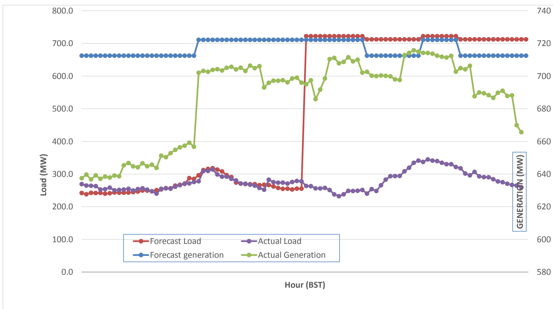
Forecast Generation & Load with Actual Generation & Load (07-Nov-2017).
