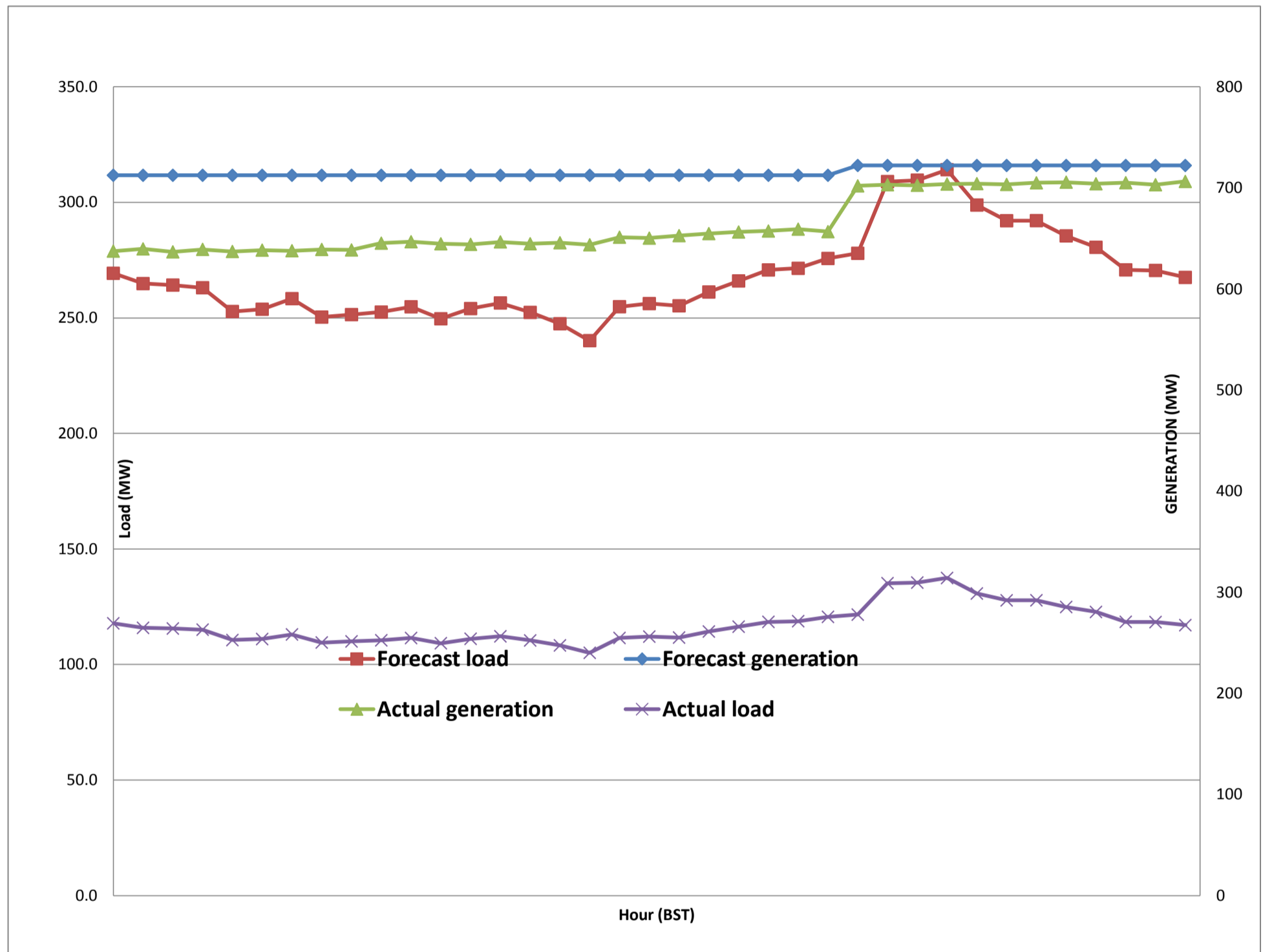
Forecast Generation & Load with Actual Generation & Load of Today from 00:00hrs to 09:00hrs(07-Nov-2017).
