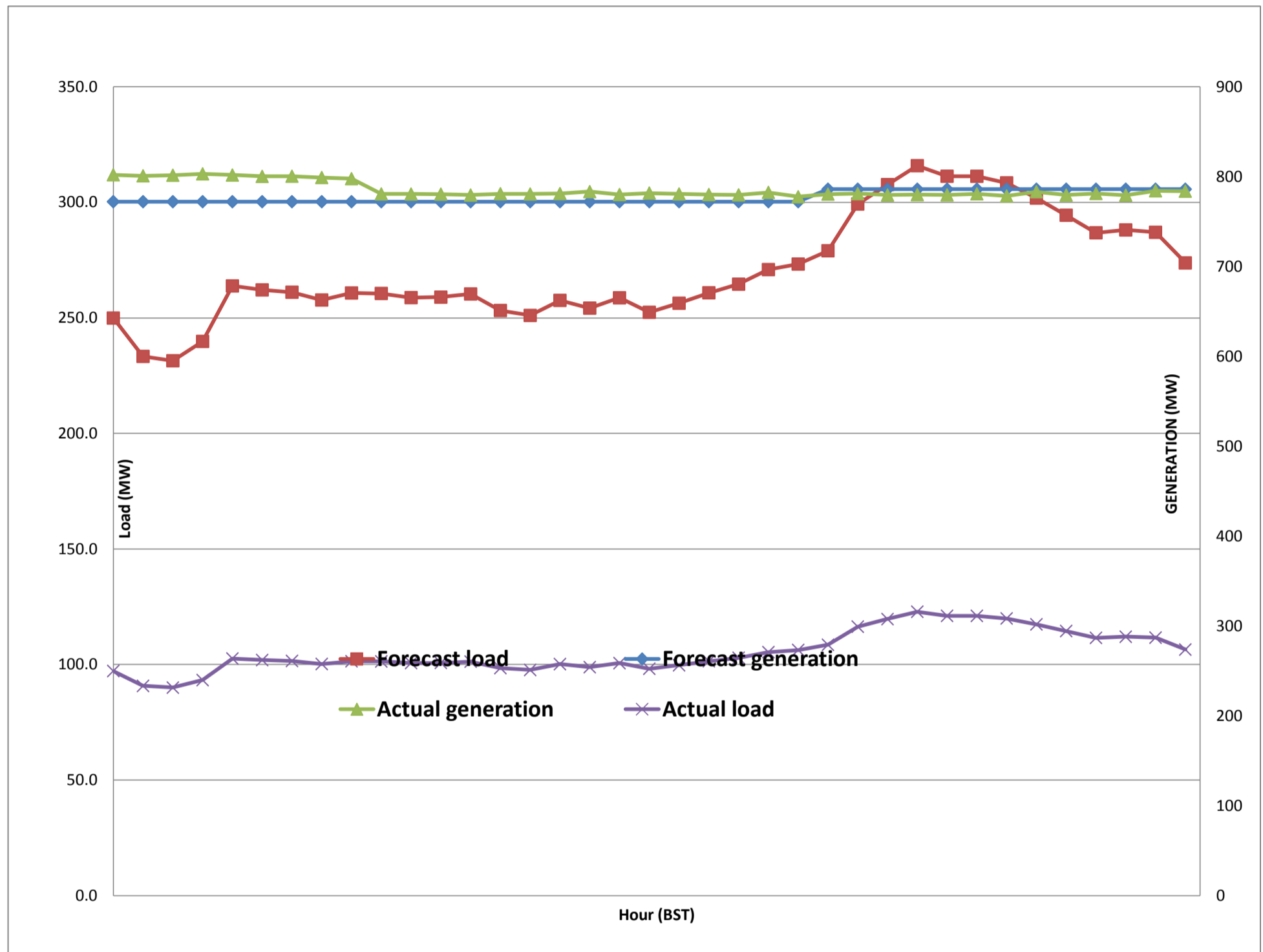
Forecast Generation & Load with Actual Generation & Load of Today from 00:00hrs to 09:00hrs(31-Oct-2017).
