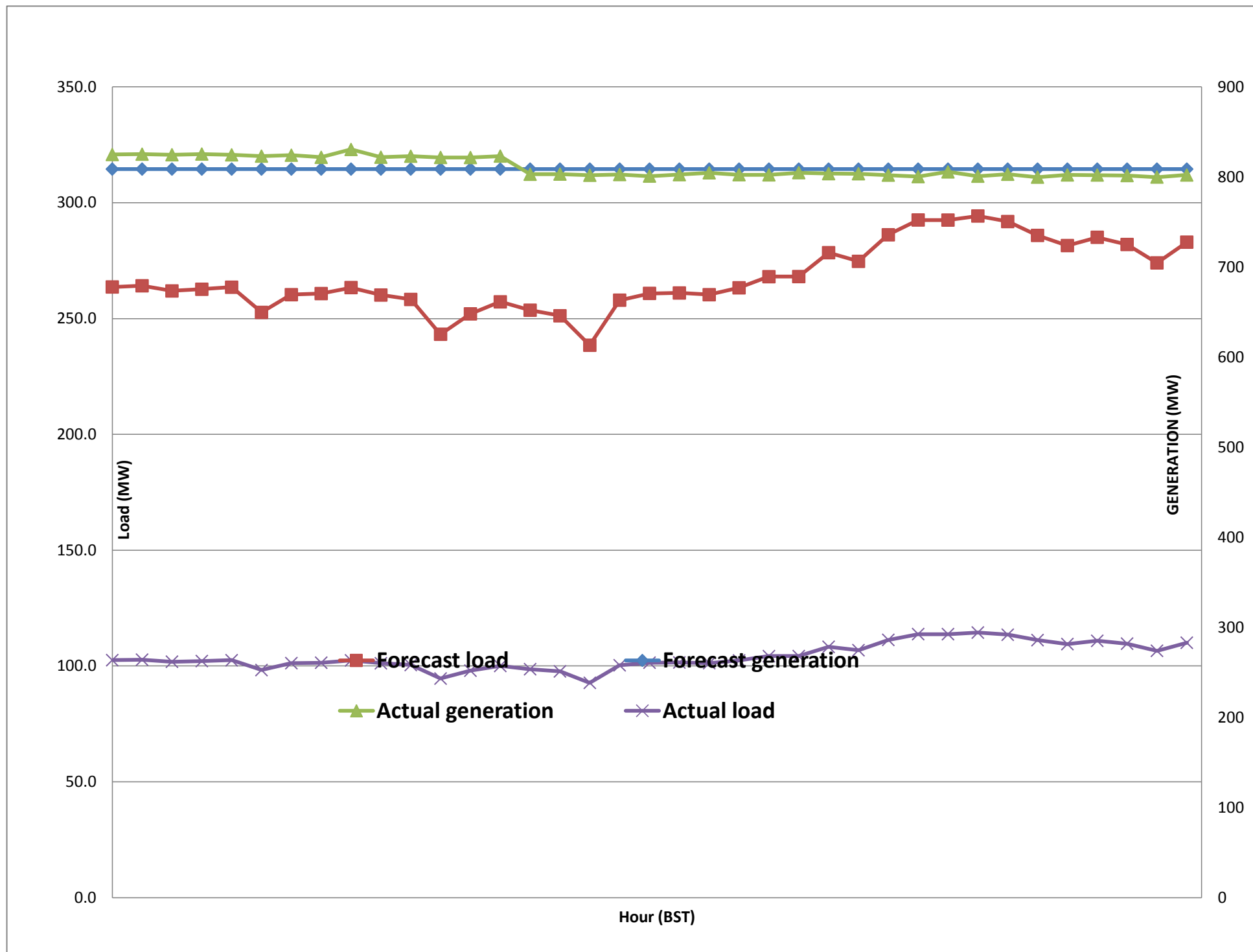
Forecast Generation & Load with Actual Generation & Load of Today from 00:00hrs to 09:00hrs(29-Oct-2017).
