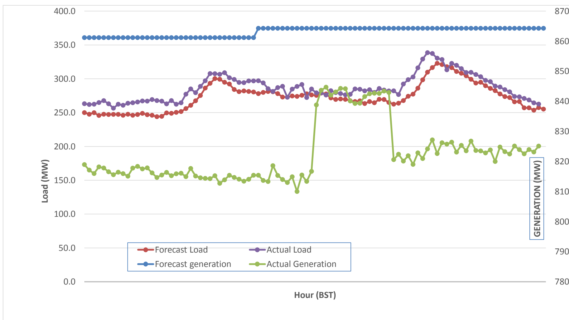
Forecast Generation & Load with Actual Generation & Load (28-Oct-2017).
