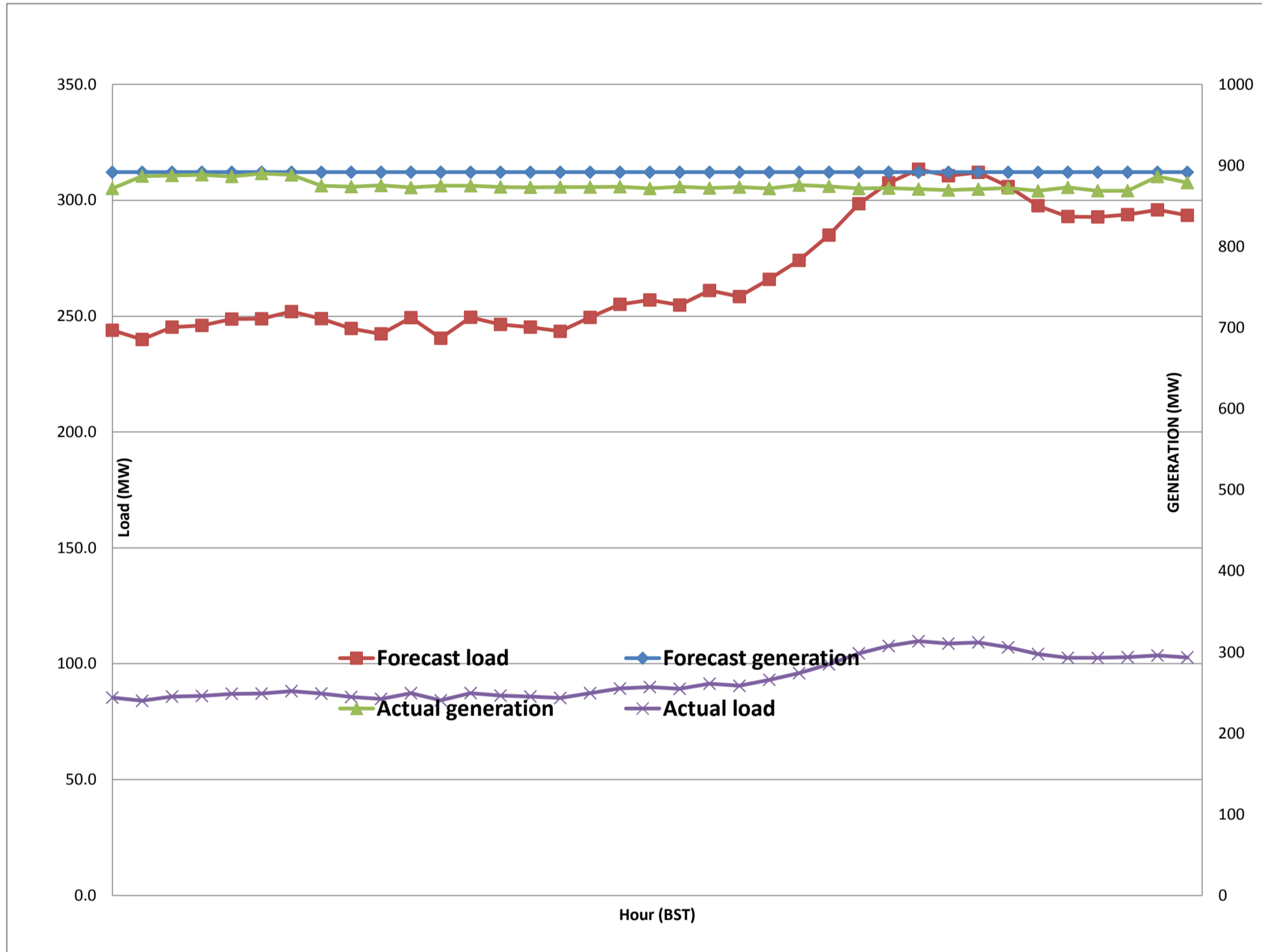
Forecast Generation & Load with Actual Generation & Load of Today from 00:00hrs to 09:00hrs(26-Oct-2017).
