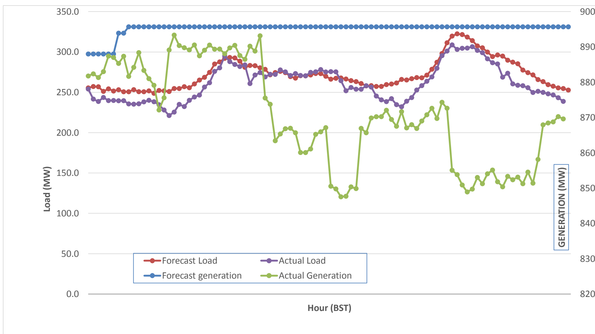
Forecast Generation & Load with Actual Generation & Load (25-Oct-2017).
