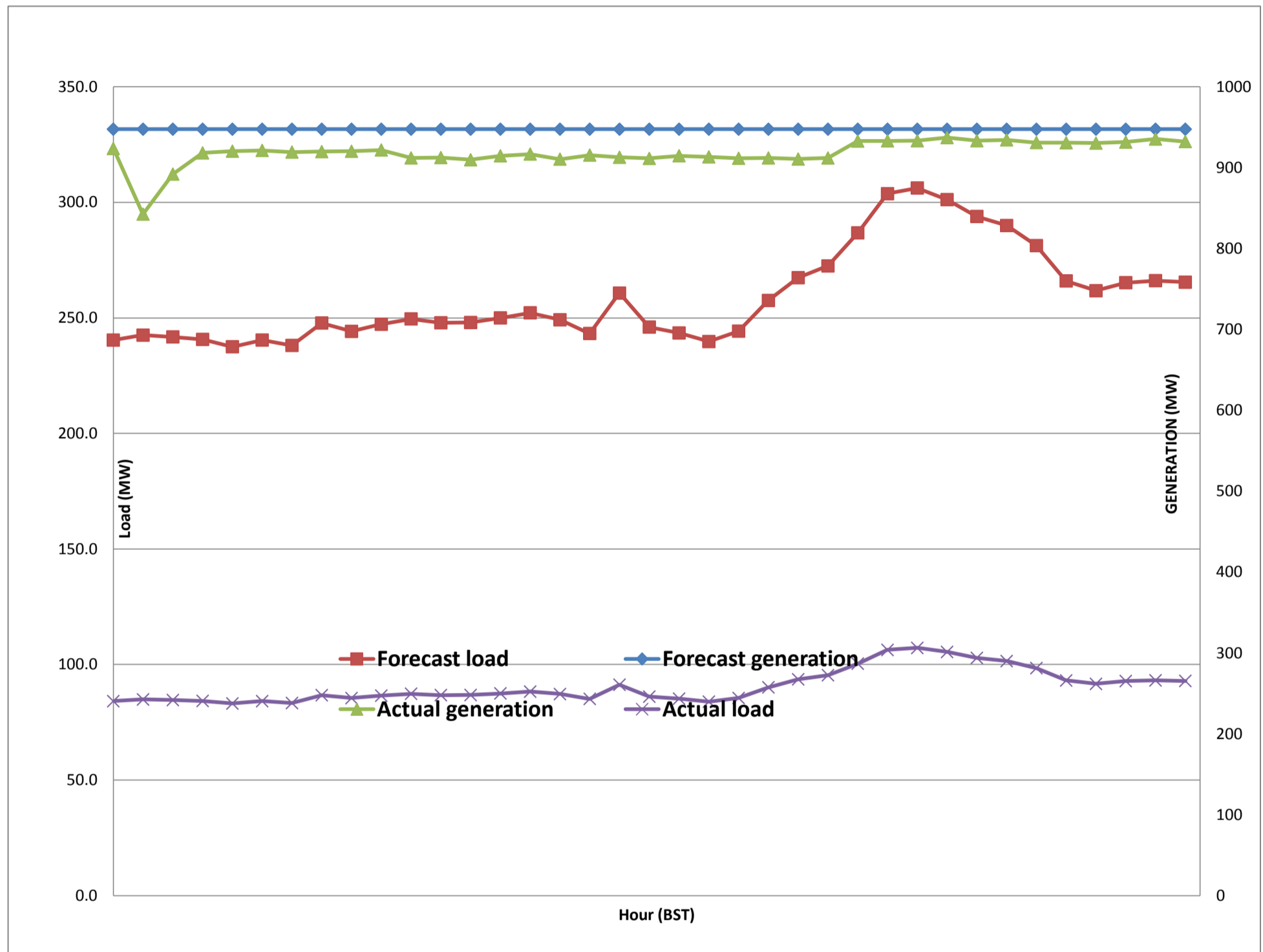
Forecast Generation & Load with Actual Generation & Load of Today from 00:00hrs to 09:00hrs(24-Oct-2017).
