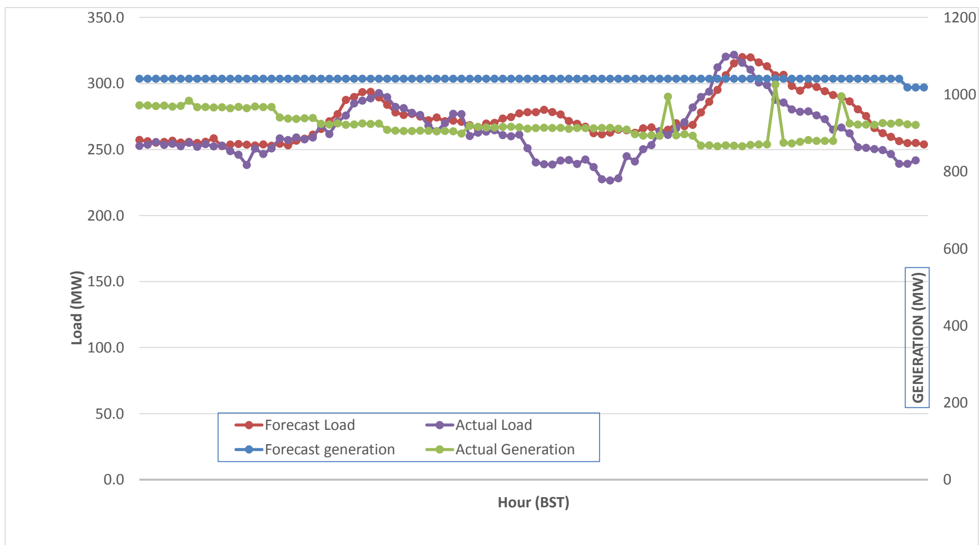
Forecast Generation & Load with Actual Generation & Load (22-Oct-2017).
