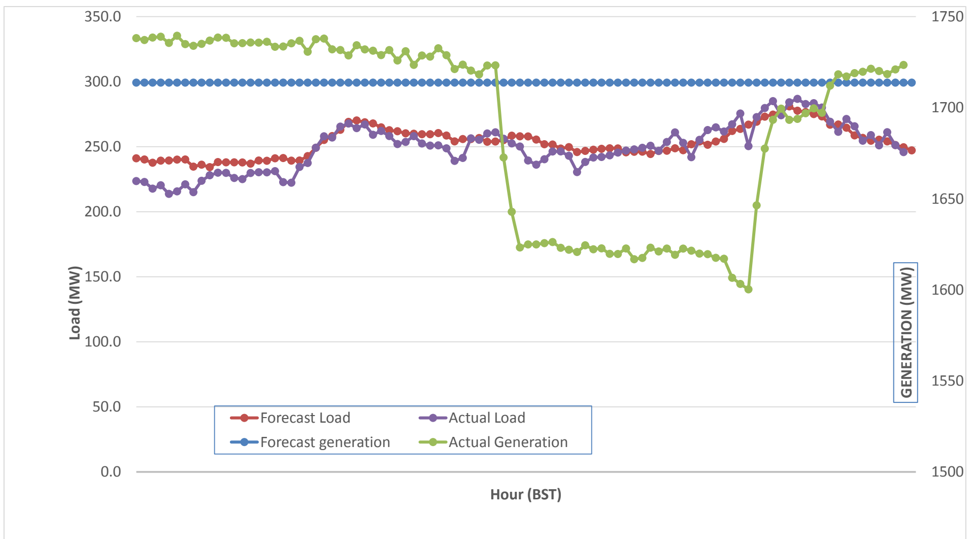
Forecast Generation & Load with Actual Generation & Load (02-Aug-2017).
