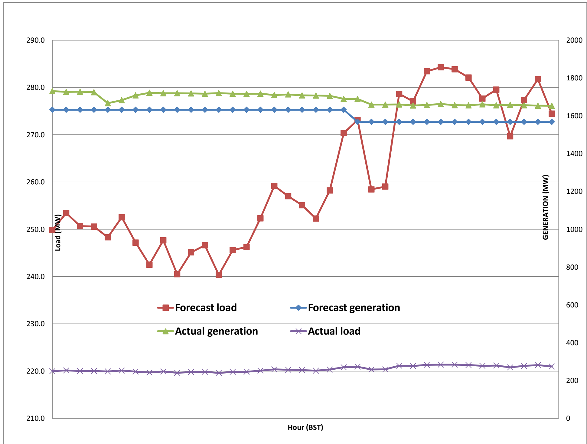
Forecast Generation & Load with Actual Generation & Load of Today from 00:00hrs to 09:00hrs(13-Jul-2017).
