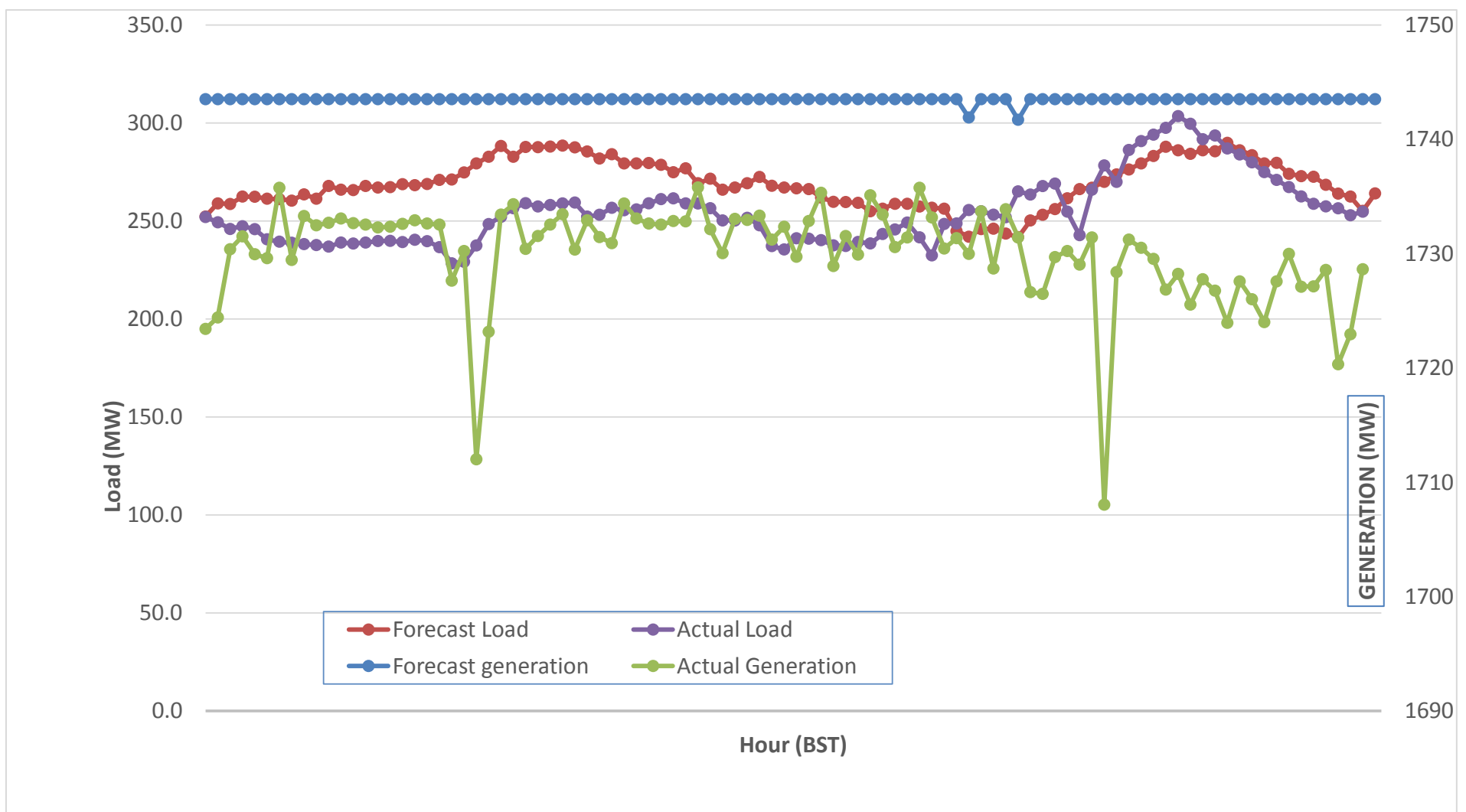
Forecast Generation & Load with Actual Generation & Load (12-Jul-2017).
