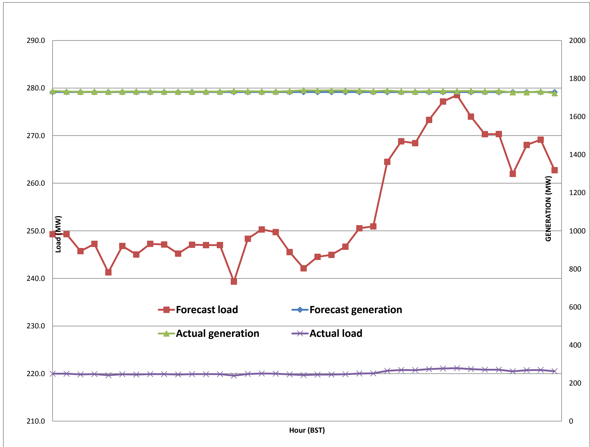
Forecast Generation & Load with Actual Generation & Load of Today from 00:00hrs to 09:00hrs(10-Jul-2017).
