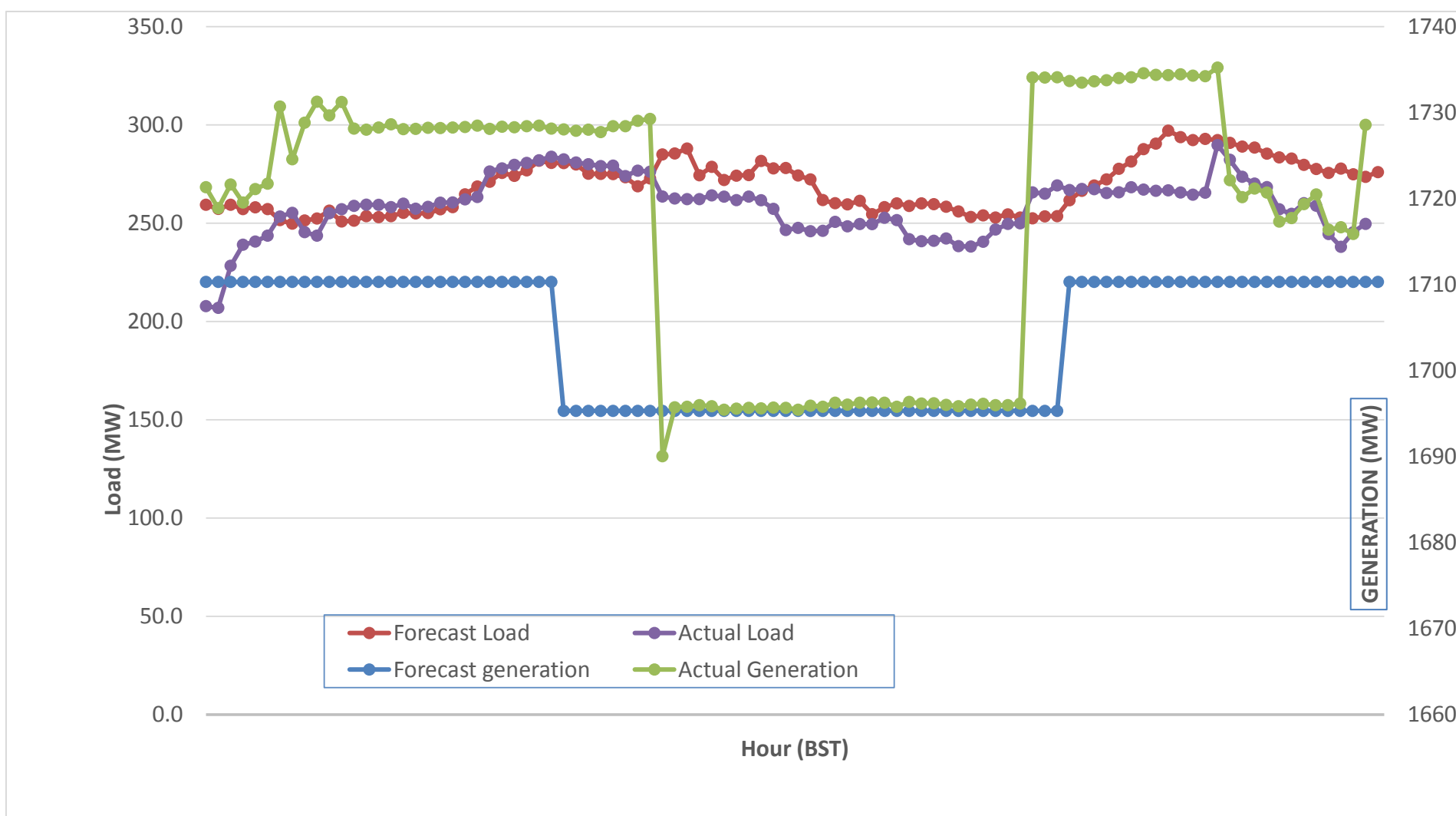
Forecast Generation & Load with Actual Generation & Load (09-Jul-2017).
