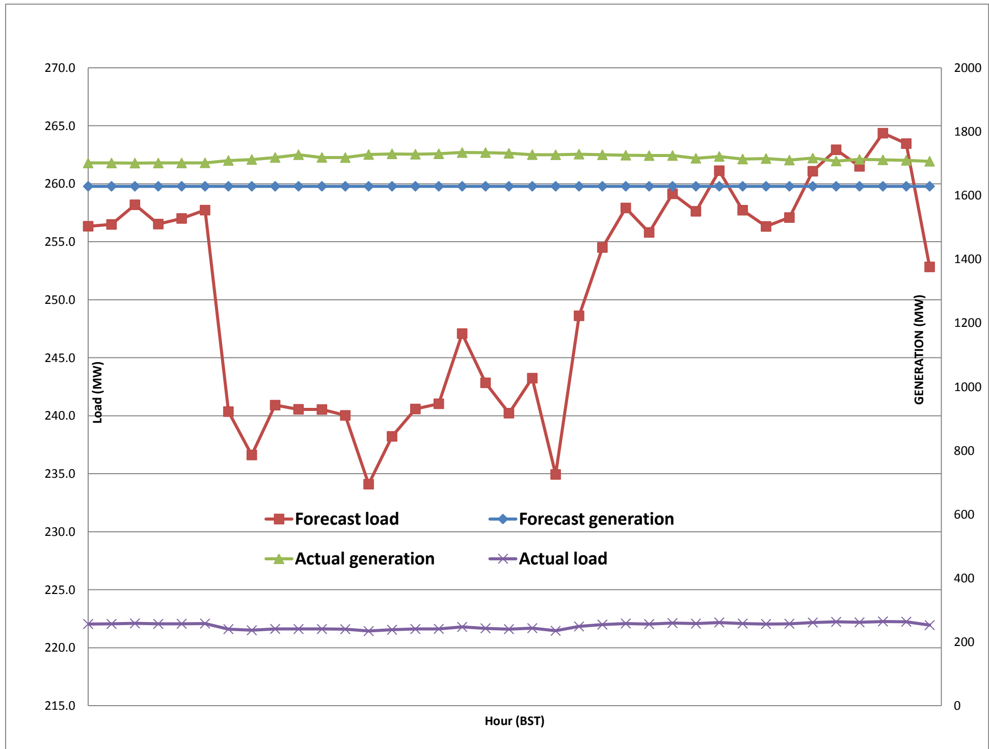
Forecast Generation & Load with Actual Generation & Load of Today from 00:00hrs to 09:00hrs(02-Jul-2017).
