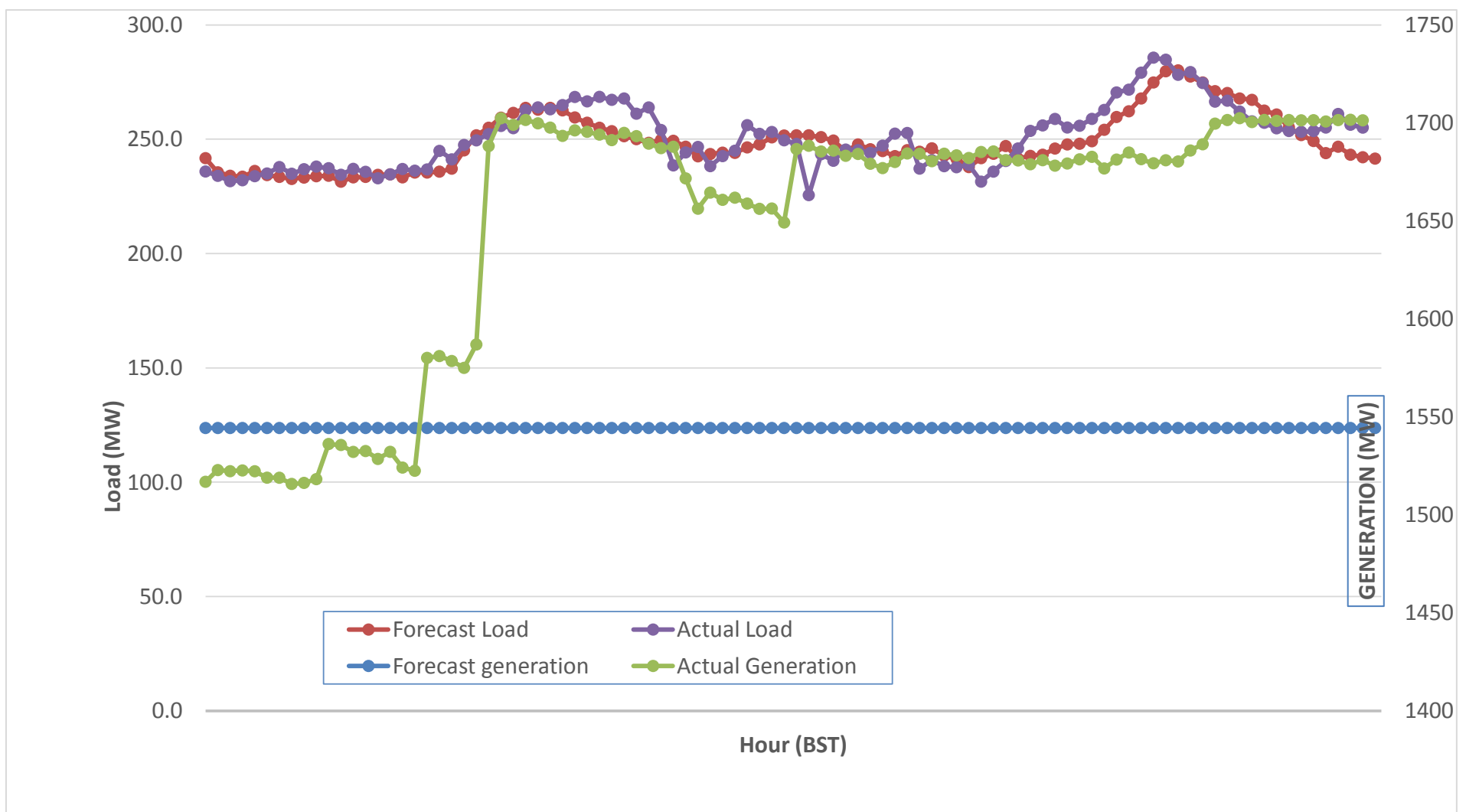
Forecast Generation & Load with Actual Generation & Load (01-Jul-2017).
